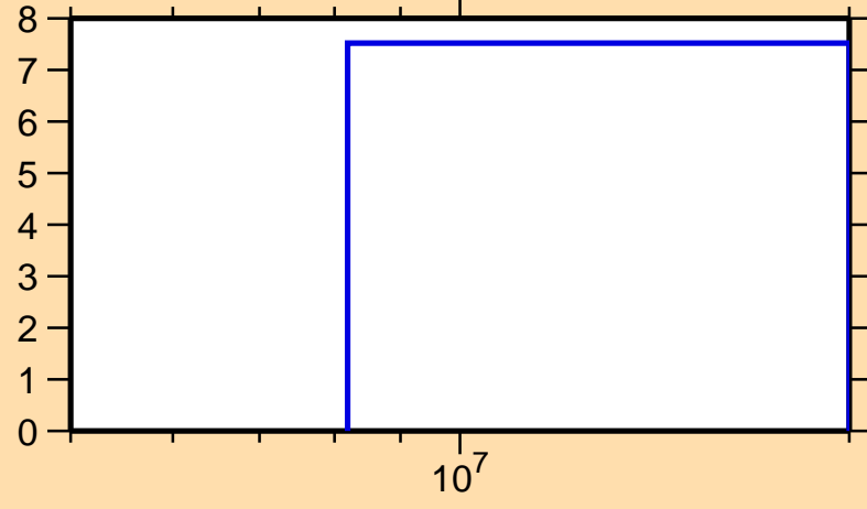
\Delta\sigma/\sigma vs. E for ^{133}\text{Sb}(n,\text{nonel.})
