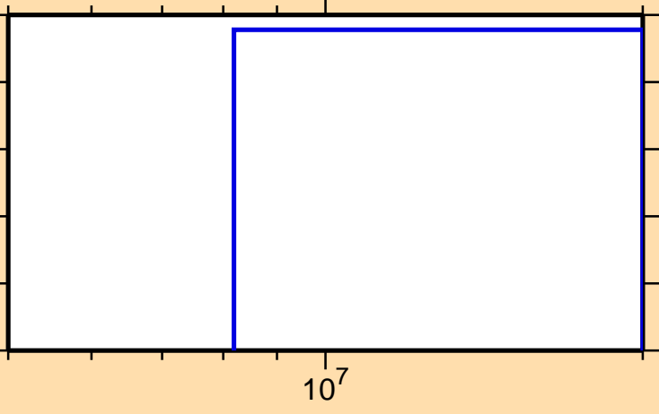
\sigma vs. E for ^{133}\text{Sb}(n,np)
