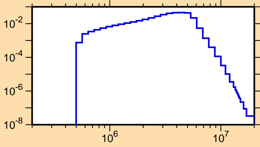
\sigma vs. E for ^{134}\text{Sb}(n,n_3)
