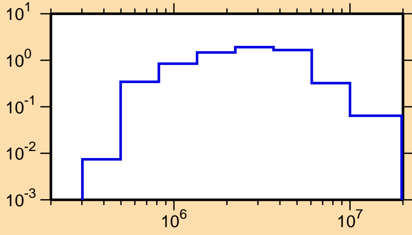
\sigma vs. E for ^{135}\text{Sb}(n,\text{inel.})
