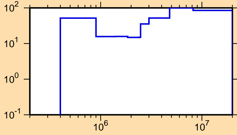
\Delta\sigma/\sigma vs. E for ^{135}\text{Sb}(n,n_1)
