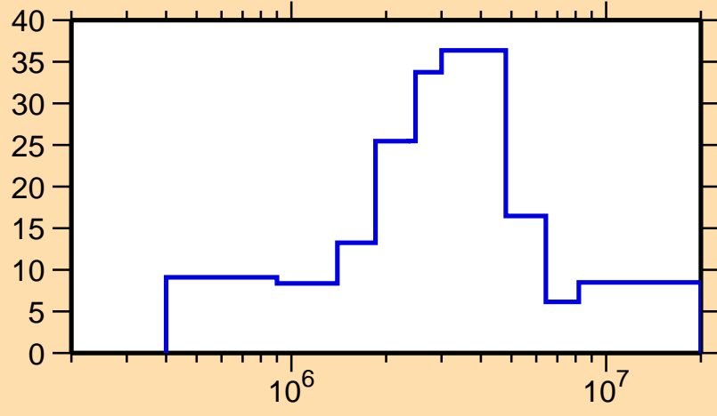
\Delta\sigma/\sigma vs. E for ^{135}\text{Sb}(n,\text{el.})
