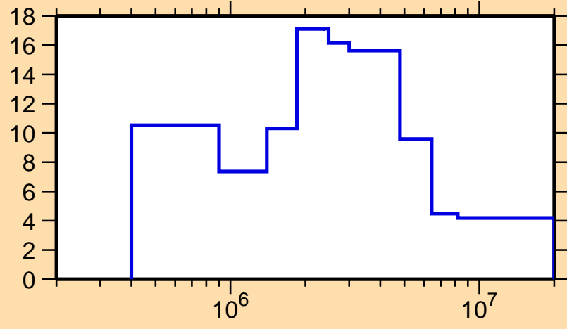
\Delta\sigma/\sigma vs. E for ^{135}\text{Sb}(n,\text{tot.})
