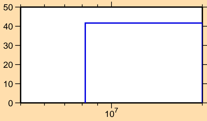
\Delta\sigma/\sigma vs. E for ^{135}\text{Sb}(n,n\text{cont.})
