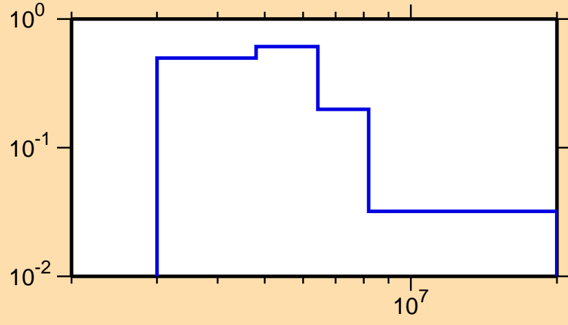
\sigma vs. E for ^{135}\text{Sb}(n,n\text{cont.})
