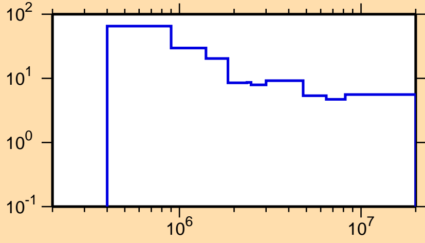
\Delta\sigma/\sigma vs. E for ^{135}\text{Sb}(n,\text{nonel.})
