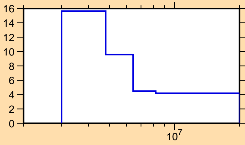
\Delta\sigma/\sigma vs. E for ^{135}\text{Sb}(n,\text{tot.})
