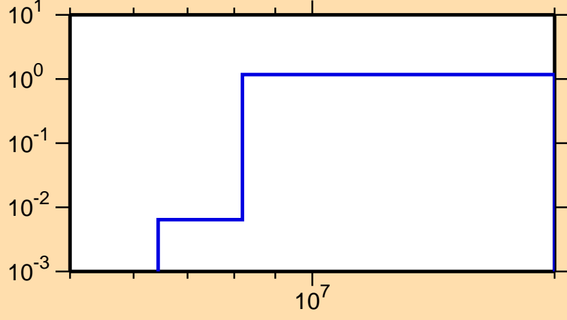
\sigma vs. E for ^{135}\text{Sb}(n,3n)
