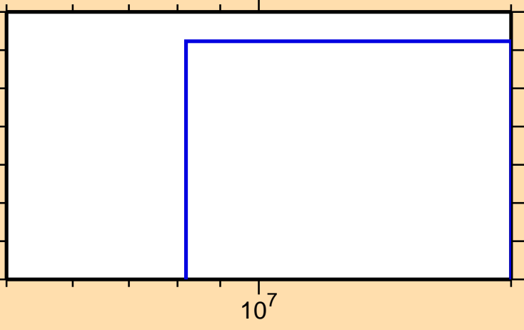
\sigma vs. E for ^{135}\text{Sb}(n,nt)
