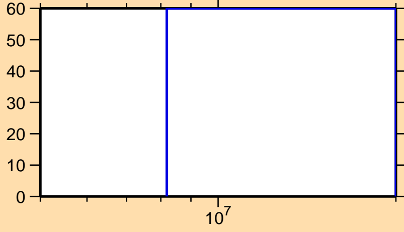
\Delta\sigma/\sigma vs. E for ^{135}\text{Sb}(n,p)
