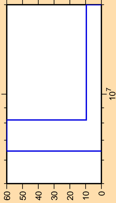
\Delta\sigma/\sigma vs. E for ^{135}\text{Sb}(n,3n)
