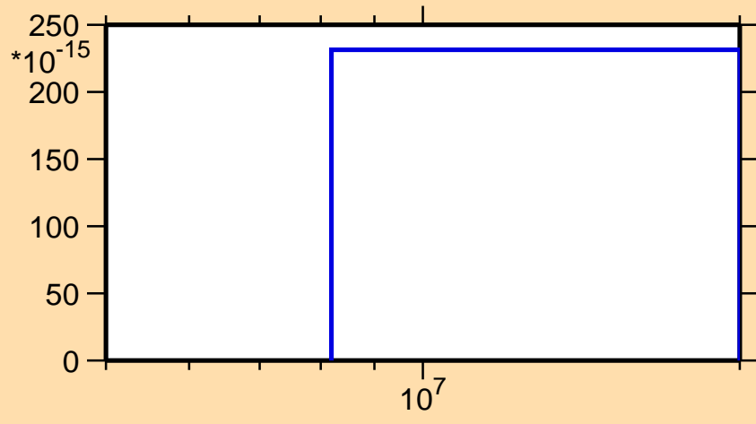
\sigma vs. E for ^{135}\text{Sb}(n,2n\alpha)
