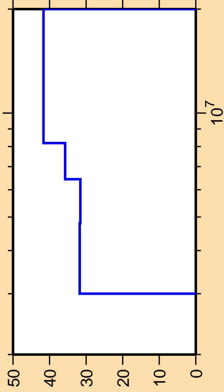
\Delta\sigma/\sigma vs. E for ^{135}\text{Sb}(n,n\text{cont.})
