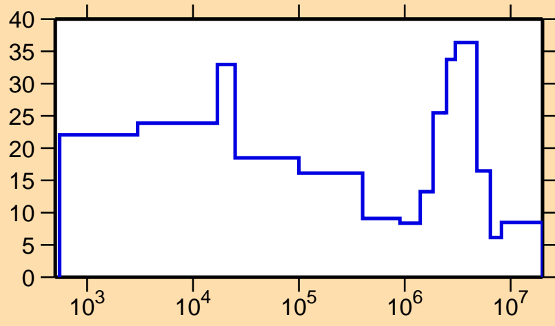
\Delta\sigma/\sigma vs. E for ^{135}\text{Sb}(n,\text{el.})
