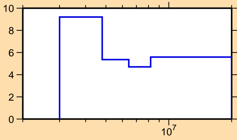
\Delta\sigma/\sigma vs. E for ^{135}\text{Sb}(n,\text{nonel.})
