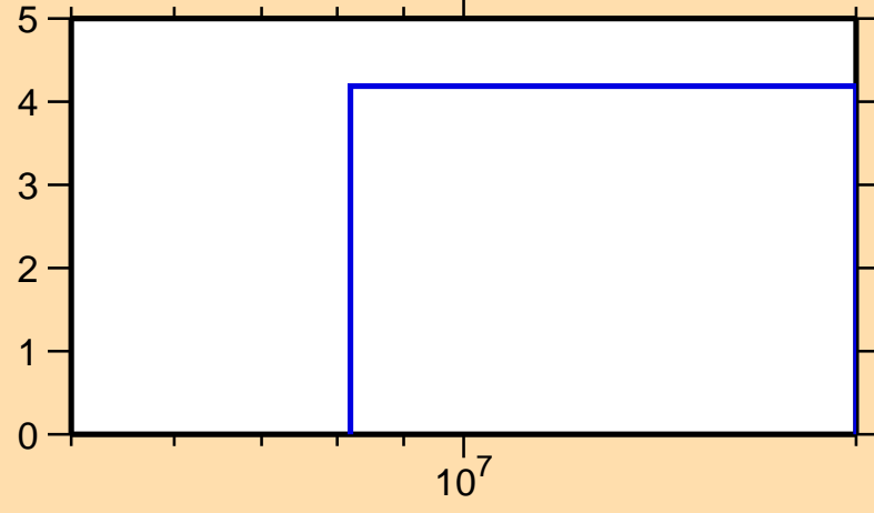
\Delta\sigma/\sigma vs. E for ^{135}\text{Sb}(n,\text{tot.})
