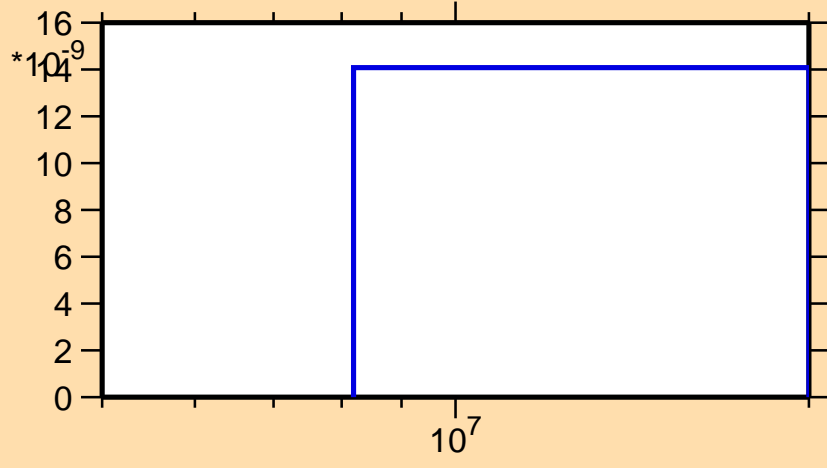
\sigma vs. E for ^{135}\text{Sb}(n,n\alpha)
