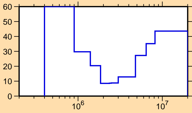
\Delta\sigma/\sigma vs. E for ^{135}\text{Sb}(n,\text{inel.})
