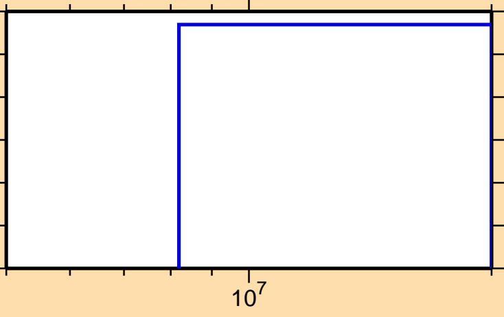
\sigma vs. E for ^{135}\text{Sb}(n,p)
