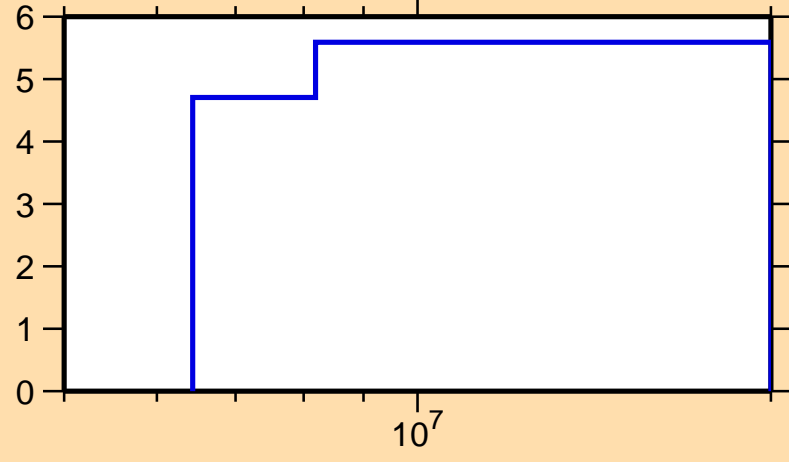
\Delta\sigma/\sigma vs. E for ^{135}\text{Sb}(n,\text{nonel.})
