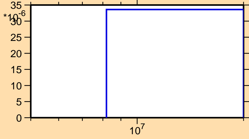
\sigma vs. E for ^{135}\text{Sb}(n,d)
