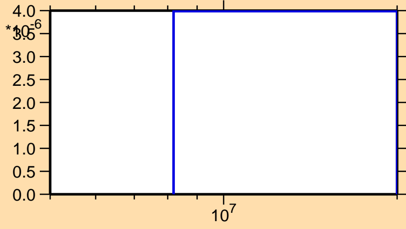
\sigma vs. E for ^{135}\text{Sb}(n,np)
