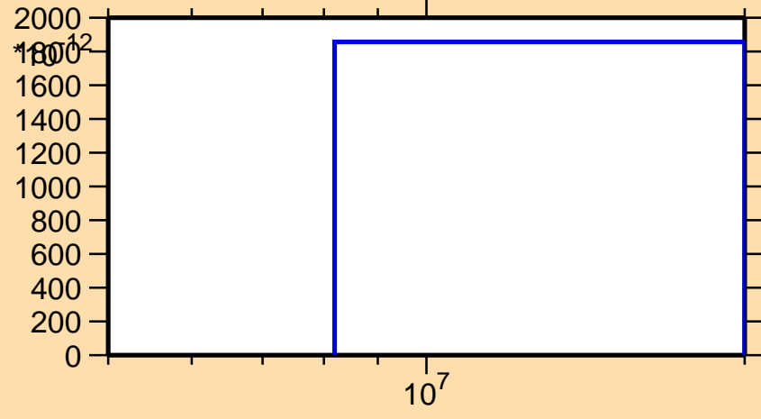
\sigma vs. E for ^{135}\text{Sb}(n,2np)
