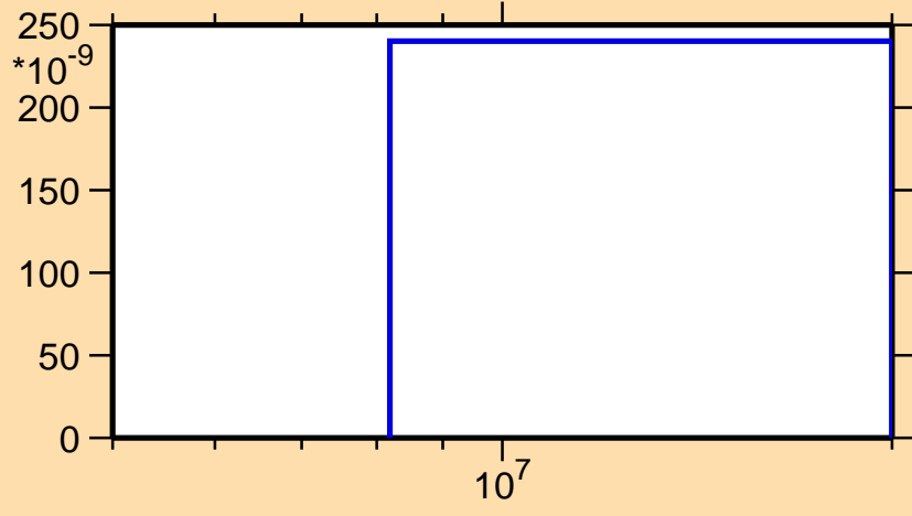
\sigma vs. E for ^{135}\text{Sb}(n,\text{nd})
