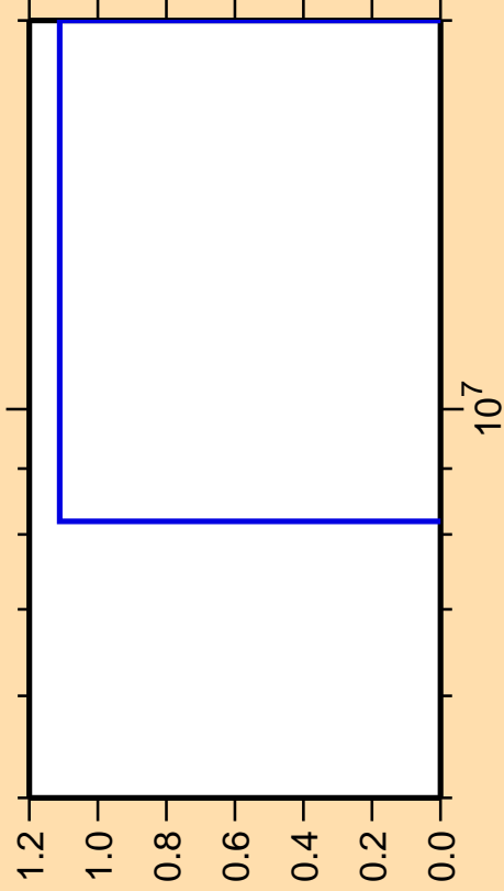
\Delta\sigma/\sigma vs. E for ^{135}\text{Sb}(n,2n\alpha)
