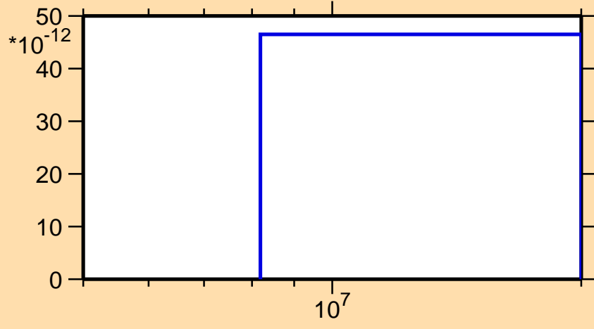
\sigma vs. E for ^{135}\text{Sb}(\text{mt } 11)
