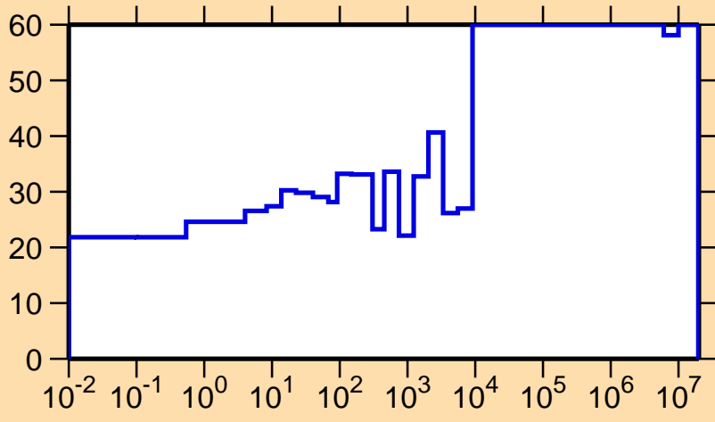
\Delta\sigma/\sigma vs. E for ^{42}\text{Sc}(n,\gamma)
