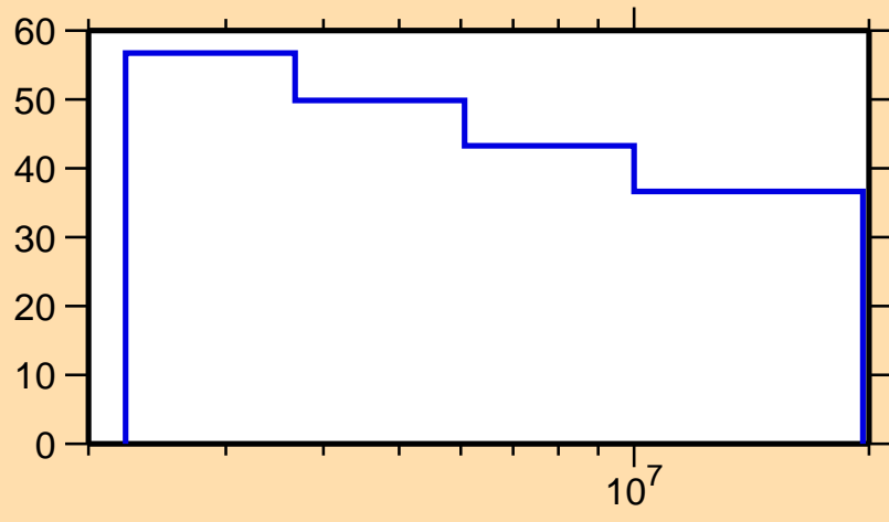
\Delta\sigma/\sigma vs. E for ^{42}\text{Sc}(n,n\text{cont.})
