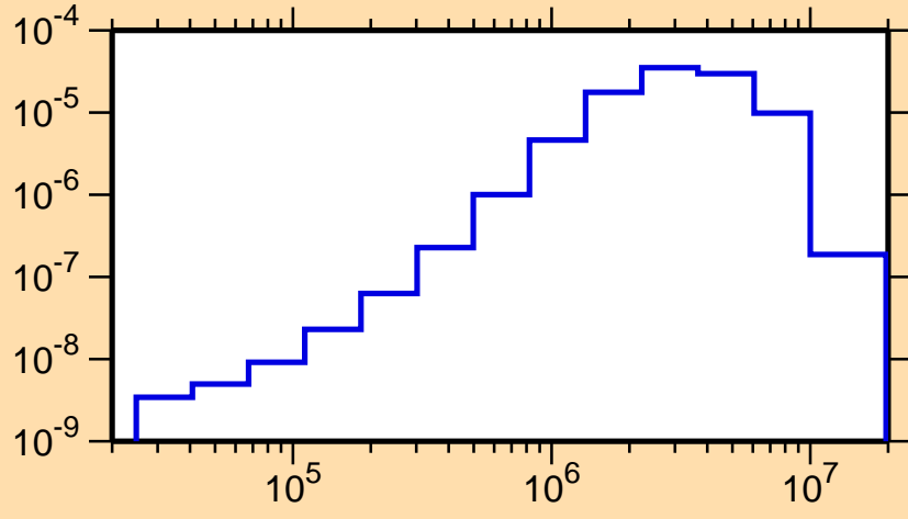
\sigma vs. E for ^{42}\text{Sc}(n,n_1)
