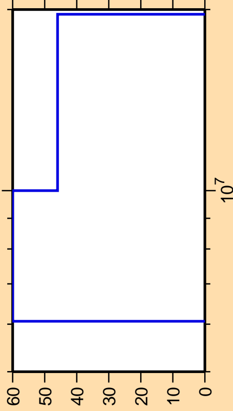
\Delta\sigma/\sigma vs. E for ^{42}\text{Sc}(n,\text{He}3)
