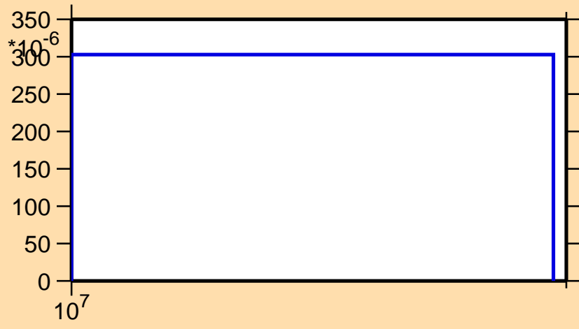
\sigma vs. E for ^{42}\text{Sc}(n,pd)
