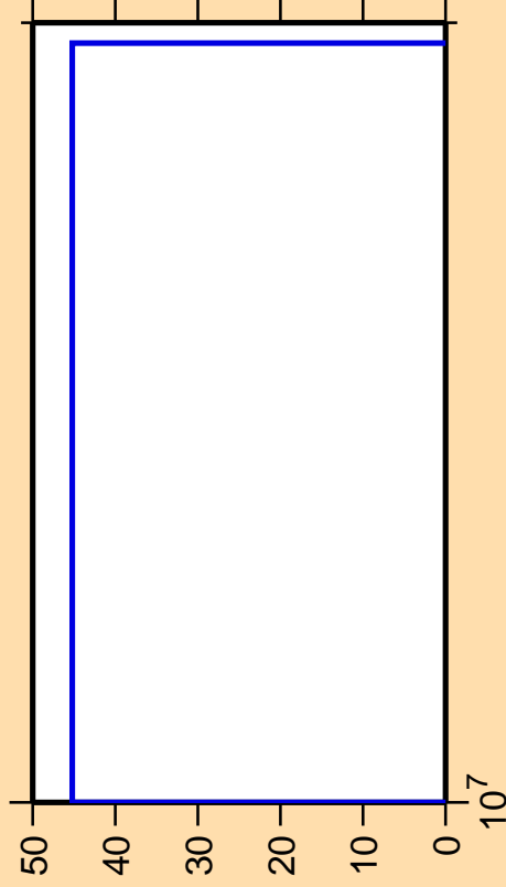
\Delta\sigma/\sigma vs. E for ^{42}\text{Sc}(n,pd)
