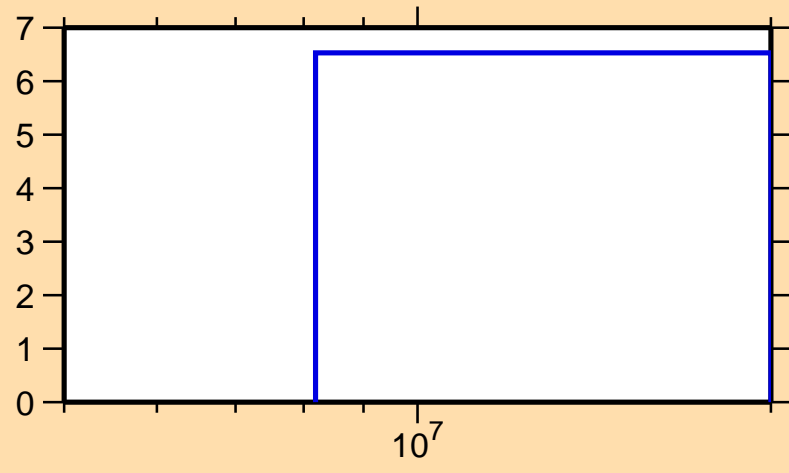
\Delta\sigma/\sigma vs. E for ^{42}\text{Sc}(n,\text{nonel.})
