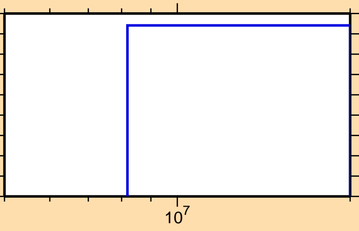
\sigma vs. E for ^{42}\text{Sc}(n,\text{pt})
