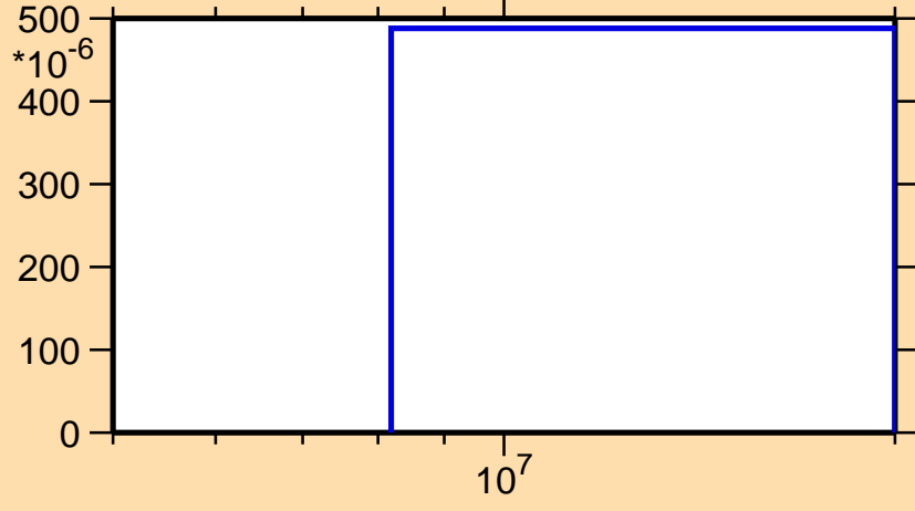
\sigma vs. E for ^{42}\text{Sc}(n,\text{nd})
