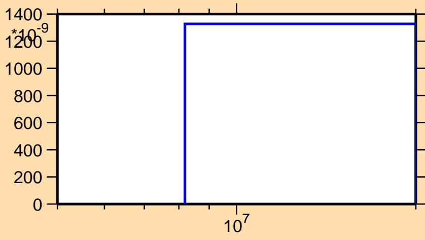
\sigma vs. E for ^{42}\text{Sc}(\text{mt } 45)
