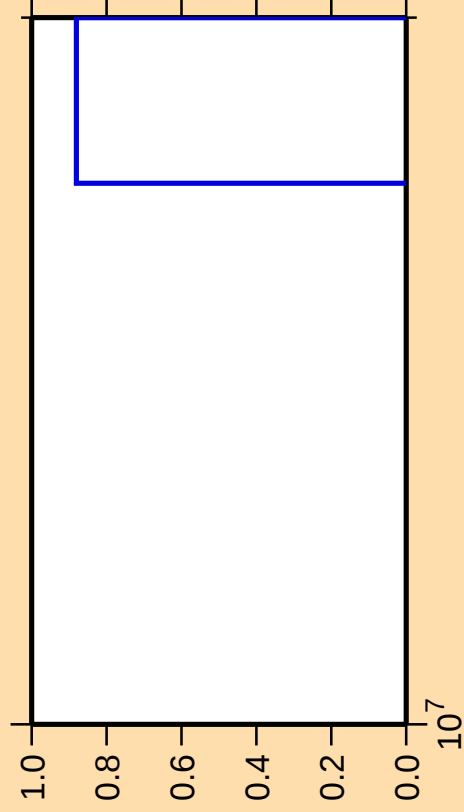
\Delta\sigma/\sigma vs. E for ^{43}\text{Sc}(\text{mt } 34)
