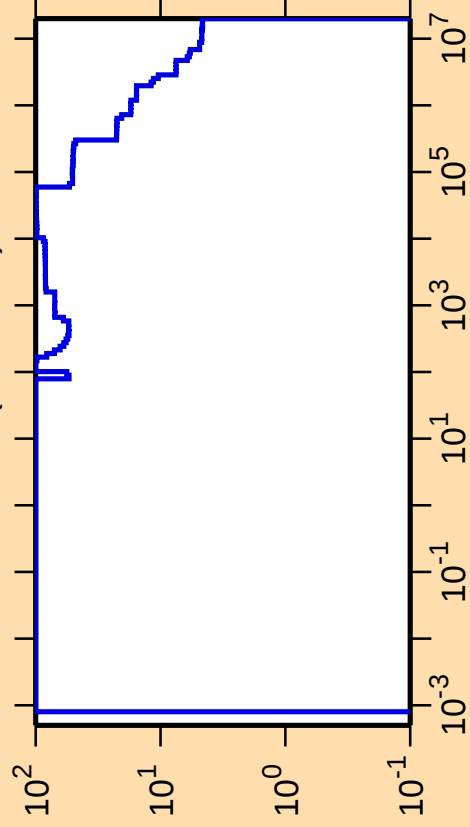
\Delta\sigma/\sigma vs. E for ^{43}\text{Sc}(n,\text{nonel.})
