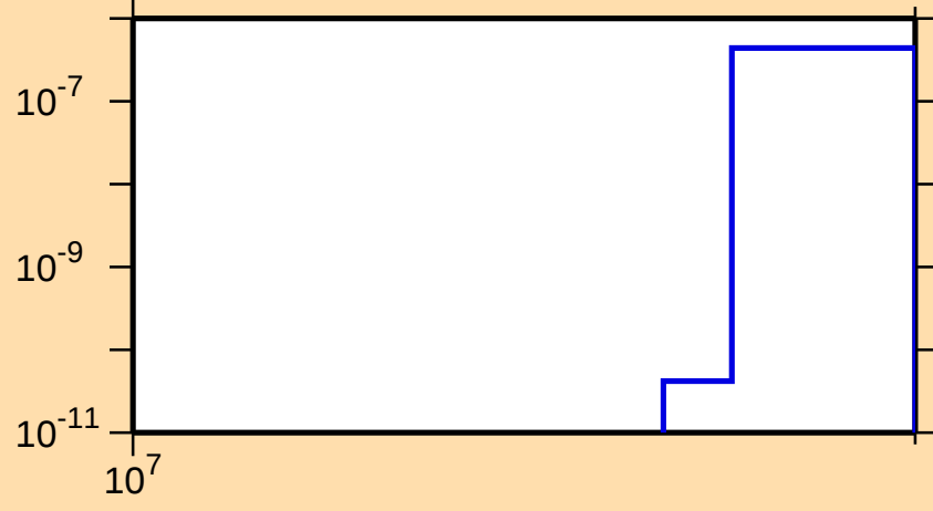
\sigma vs. E for ^{43}\text{Sc}(n,nt)
