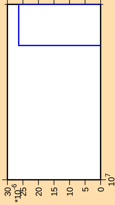
\Delta\sigma/\sigma vs. E for ^{43}\text{Sc}(n,2n\alpha)
