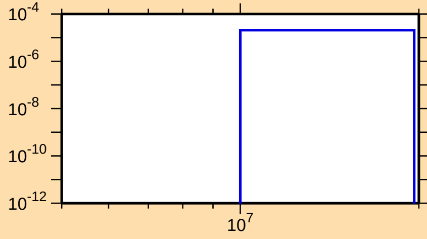
\sigma vs. E for ^{43}\text{Sc}(n,\text{He3})
