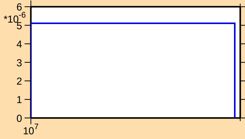
\sigma vs. E for ^{43}\text{Sc}(n,\text{nd})
