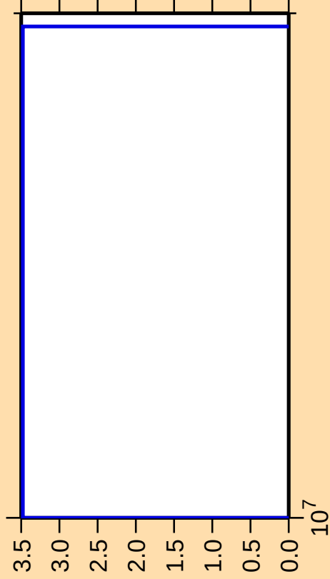
\Delta\sigma/\sigma vs. E for ^{43}\text{Sc}(\text{n},\text{pt})
