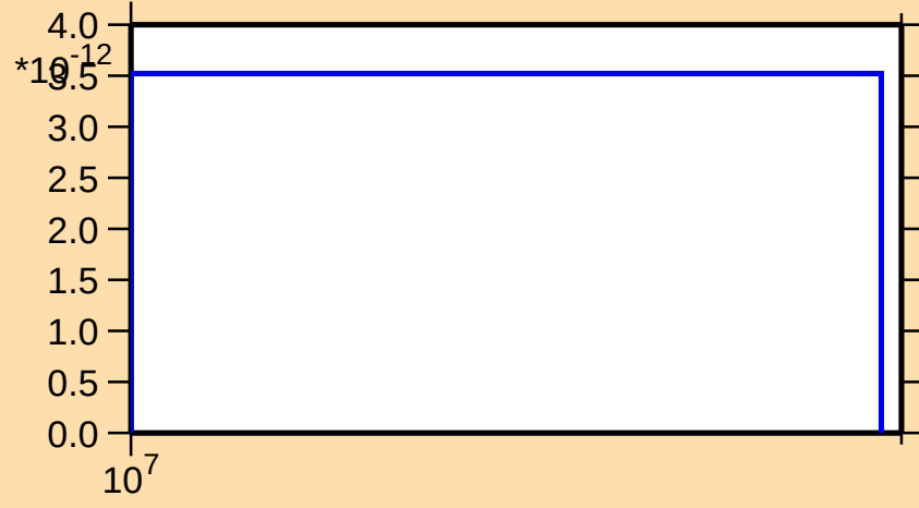
\sigma vs. E for ^{43}\text{Sc}(\text{n},\text{pt})
