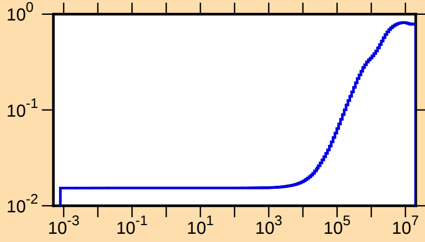
\mu vs. E for ^{44}\text{Sc}(\text{mt251})
