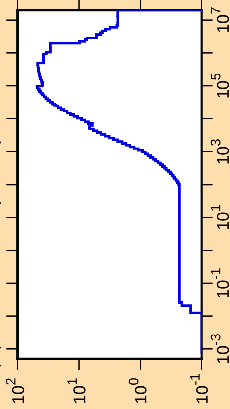
\Delta\mu/\mu vs. E for ^{44}\text{Sc}(\text{mt251})
