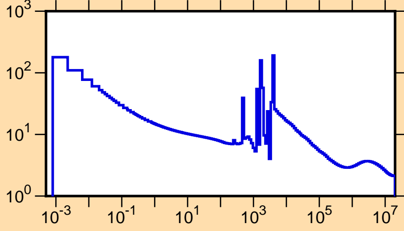
\sigma vs. E for ^{44}\text{Sc}(n,\text{tot.})
