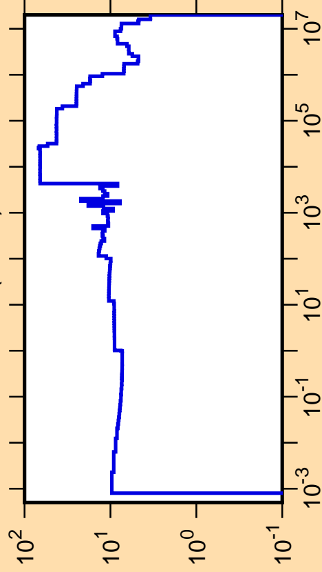
\Delta\sigma/\sigma vs. E for ^{44}\text{Sc}(n,\text{tot.})
