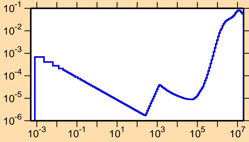
\sigma vs. E for ^{45}\text{Sc}(n,p)
