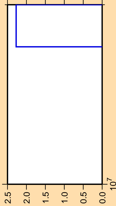
\Delta\sigma/\sigma vs. E for ^{45}\text{Sc}(n,pd)
