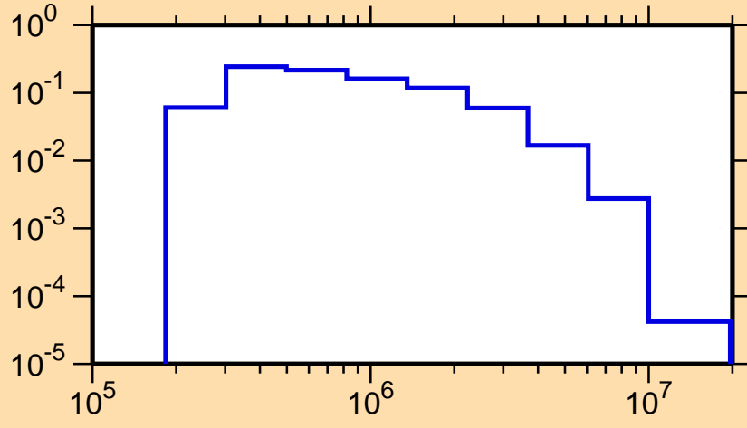
\sigma vs. E for ^{46}\text{Sc}(n,n_3)
