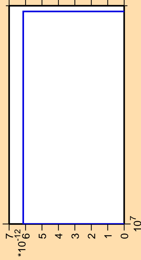
\Delta\sigma/\sigma vs. E for ^{46}\text{Sc} (mt 45)
