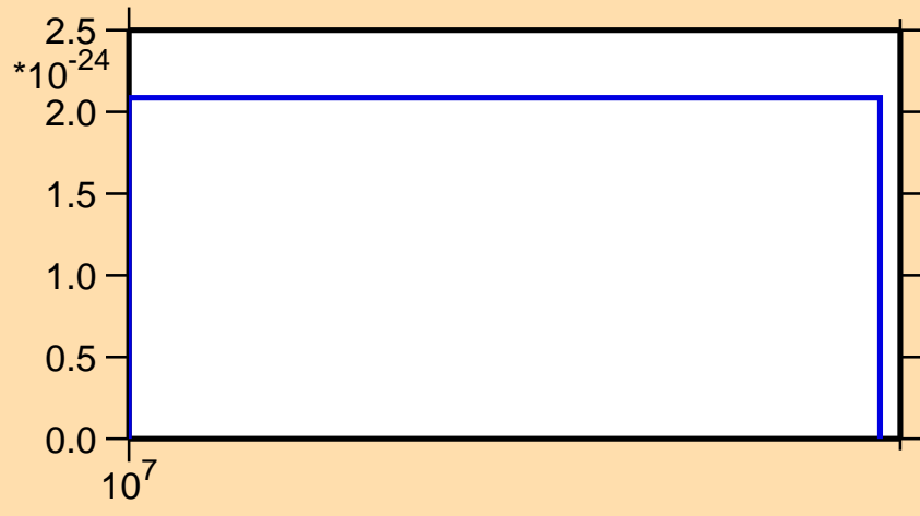
\sigma vs. E for ^{46}\text{Sc} (mt 45)
