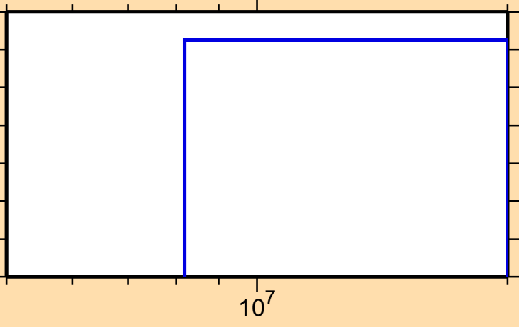
\sigma vs. E for ^{46}\text{Sc}(n,\text{pd})
