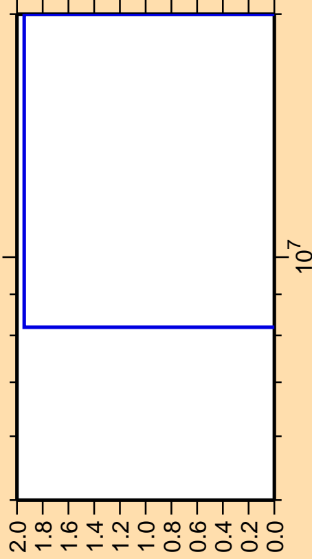
\Delta\sigma/\sigma vs. E for ^{46}\text{Sc}(n,2n\alpha)
