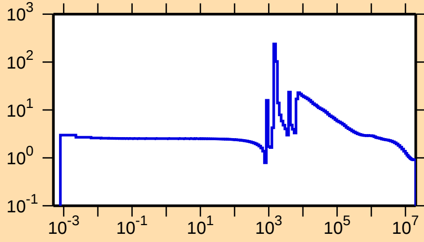
\sigma vs. E for ^{47}\text{Sc}(n,\text{el.})
