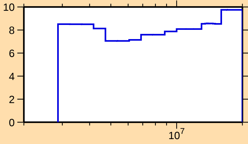
\Delta\sigma/\sigma vs. E for ^{47}\text{Sc}(n,\text{nonel.})
