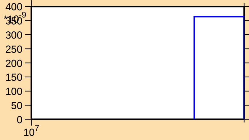
\sigma vs. E for ^{47}\text{Sc}(n,3n)
