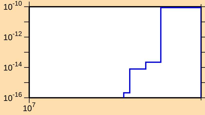
\sigma vs. E for ^{47}\text{Sc}(n,\text{He3})
