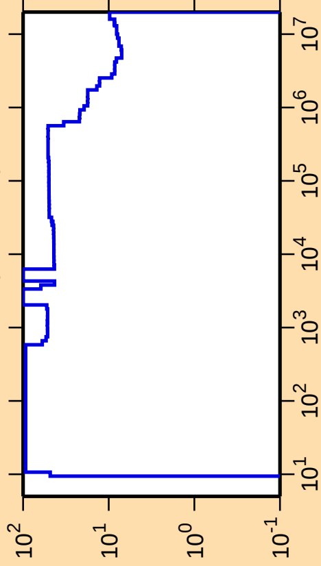
\Delta\sigma/\sigma vs. E for ^{47}\text{Sc}(n,\text{nonel.})
