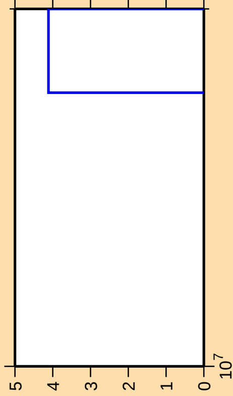
\Delta\sigma/\sigma vs. E for ^{47}\text{Sc}(n,2np)
