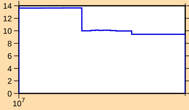
\Delta\sigma/\sigma vs. E for ^{47}\text{Sc}(n,\text{el.})
