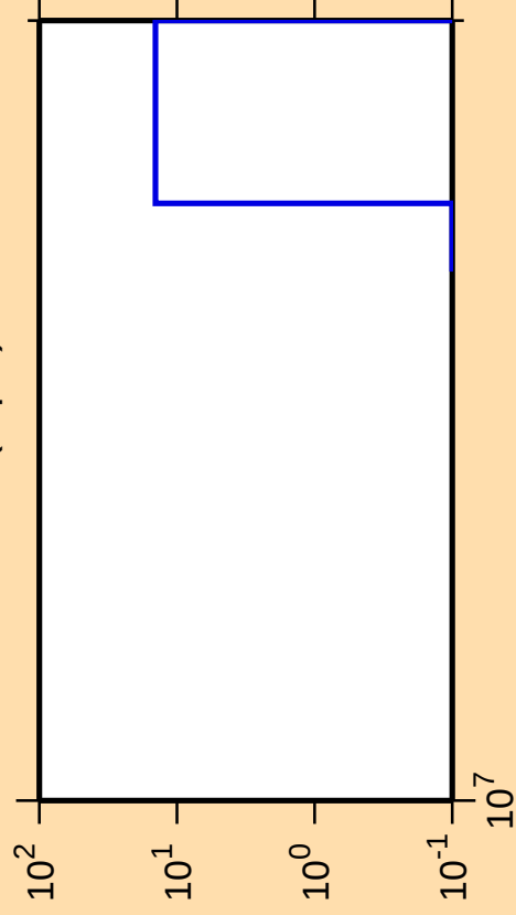
\Delta\sigma/\sigma vs. E for ^{47}\text{Sc}(n,p\alpha)
