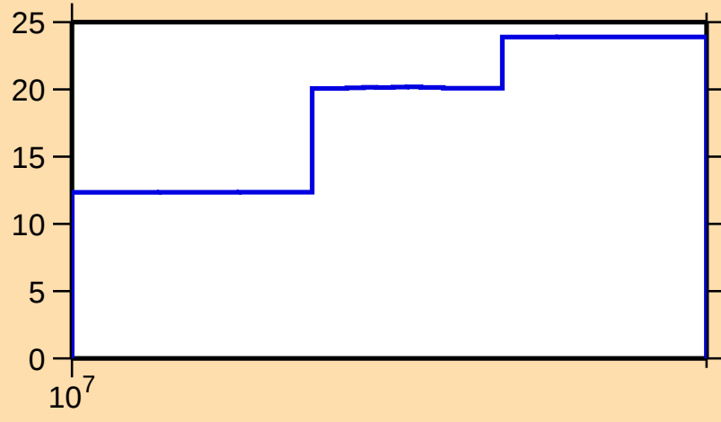
\Delta\sigma/\sigma vs. E for ^{47}\text{Sc}(n,\text{inel.})
