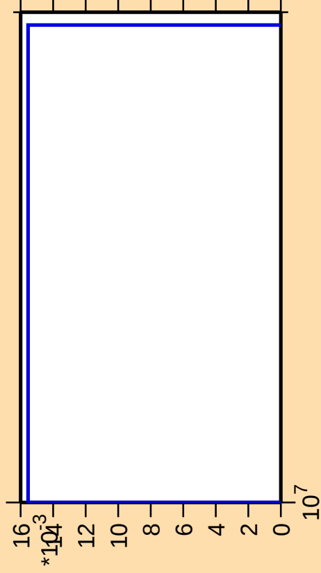
\Delta\sigma/\sigma vs. E for ^{47}\text{Sc}(n,2np)
