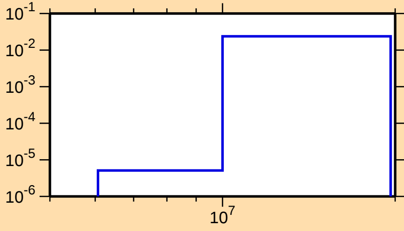
\sigma vs. E for ^{47}\text{Sc}(n,np)
