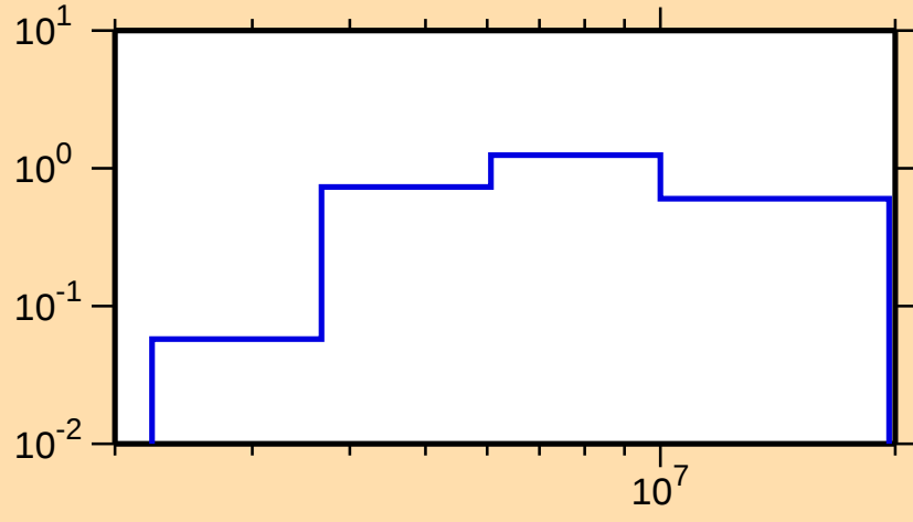
\sigma vs. E for ^{47}\text{Sc}(n,n\text{cont.})
