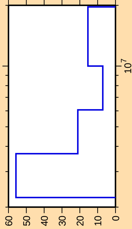
\Delta\sigma/\sigma vs. E for ^{47}\text{Sc}(\text{n},\text{ncont.})
