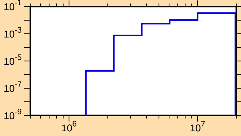
\sigma vs. E for ^{47}\text{Sc}(n,p)
