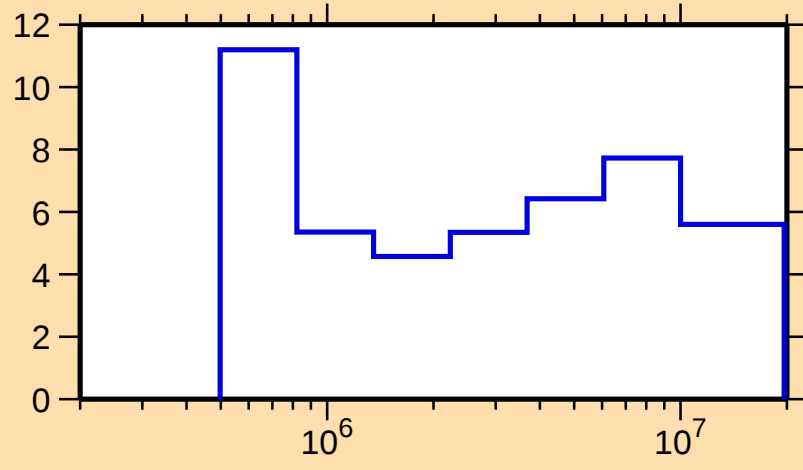
\Delta\sigma/\sigma vs. E for ^{47}\text{Sc}(n,\text{tot.})
