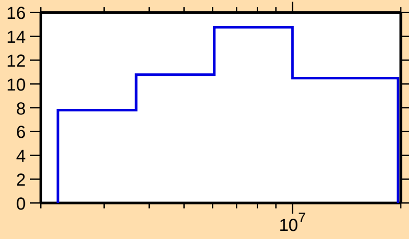
\Delta\sigma/\sigma vs. E for ^{47}\text{Sc}(\text{n},\text{el.})
