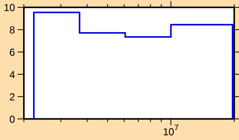
\Delta\sigma/\sigma vs. E for ^{47}\text{Sc}(\text{n},\text{nonel.})
