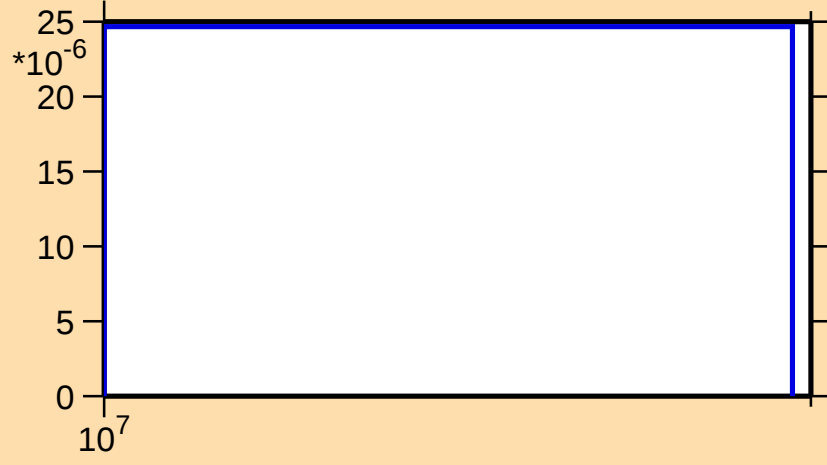
\sigma vs. E for ^{47}\text{Sc}(n,t)
