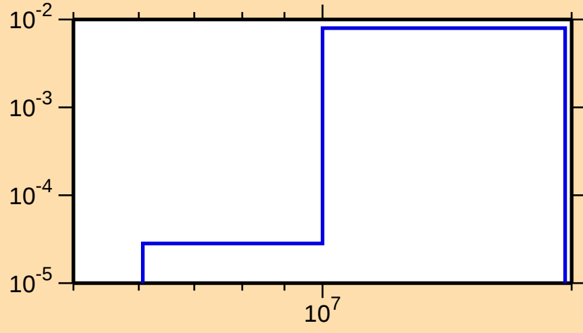
\sigma vs. E for ^{47}\text{Sc}(n,d)
