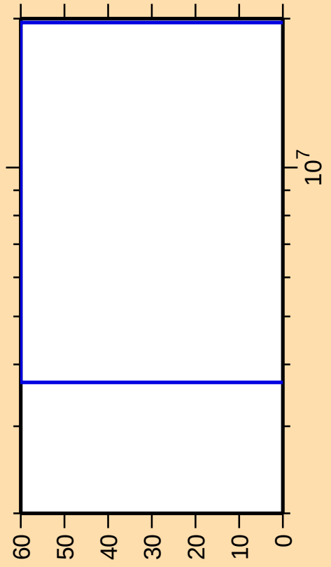
\Delta\sigma/\sigma vs. E for ^{47}\text{Sc}(n,\alpha)
