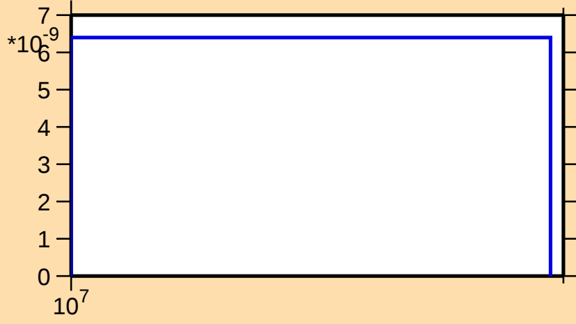
\sigma vs. E for ^{47}\text{Sc}(n,\text{nd})
