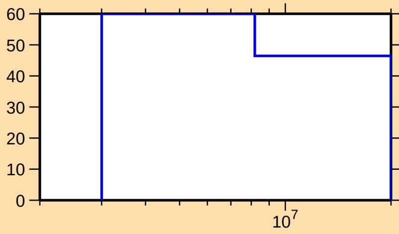
\Delta\sigma/\sigma vs. E for ^{47}\text{Sc}(n,p)
