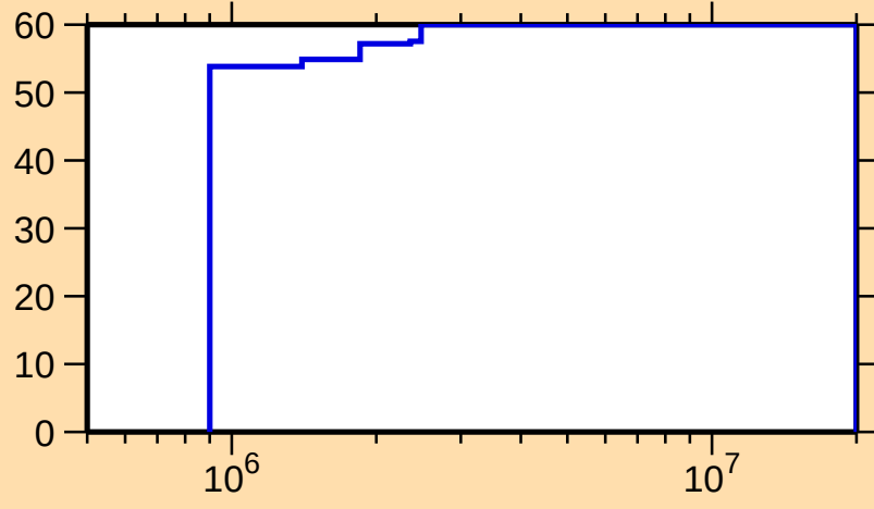
\Delta\sigma/\sigma vs. E for ^{47}\text{Sc}(n,\gamma)
