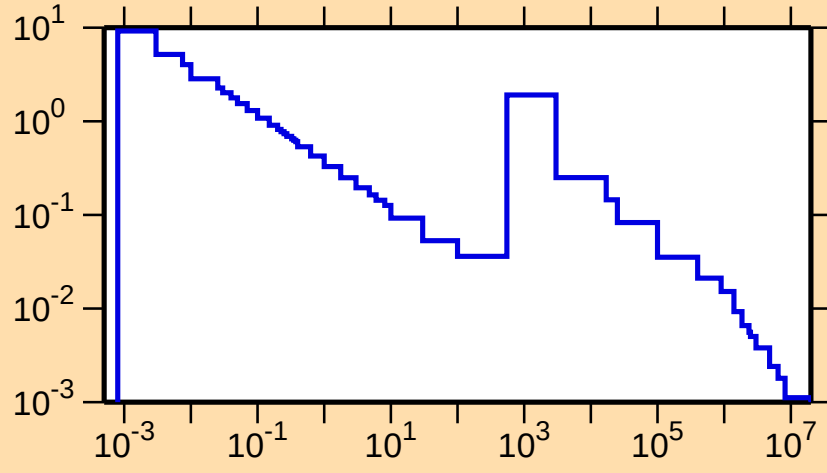
\sigma vs. E for ^{47}\text{Sc}(n,\gamma)
