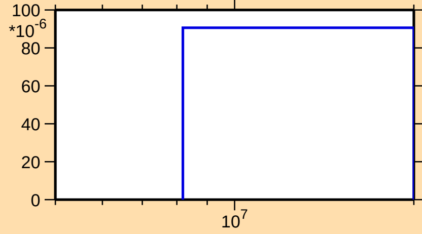
\sigma vs. E for ^{47}\text{Sc}(n,n\alpha)
