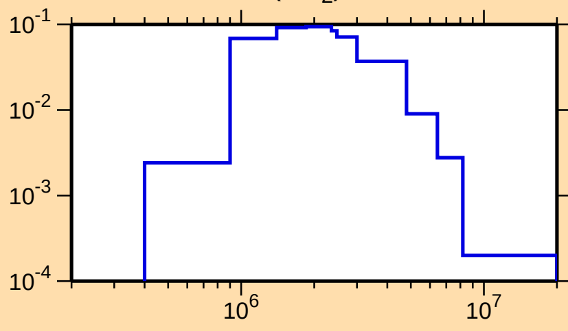
\sigma vs. E for ^{47}\text{Sc}(n,n_2)
