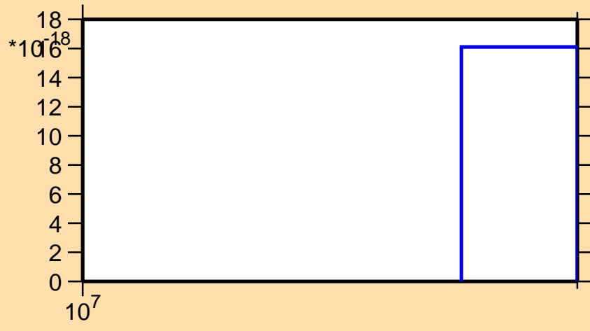
\sigma vs. E for ^{49}\text{Sc}(n,\text{He}3)
