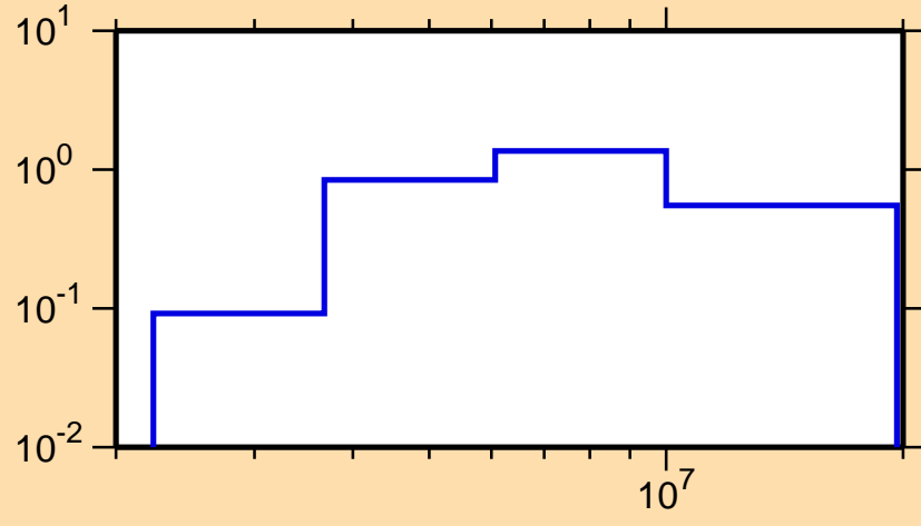
\sigma vs. E for ^{49}\text{Sc}(n,\text{inel.})
