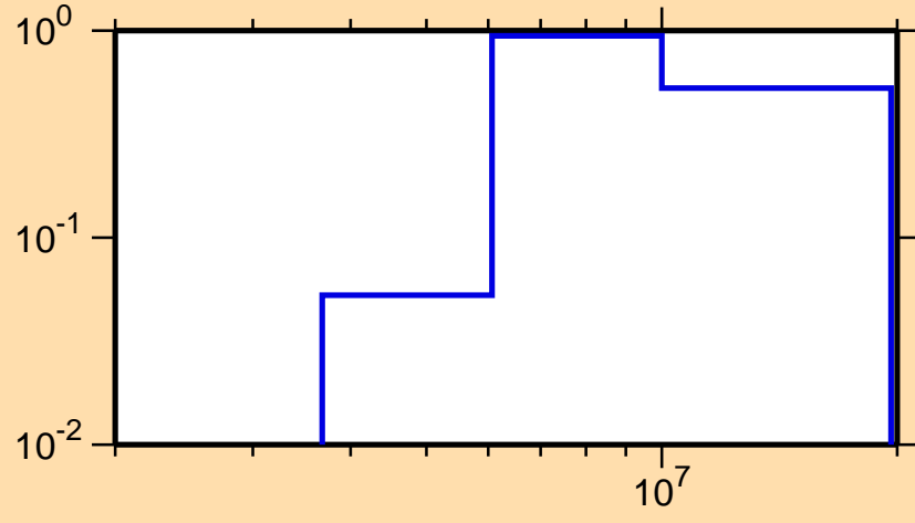
\sigma vs. E for ^{49}\text{Sc}(n,n\text{cont.})
