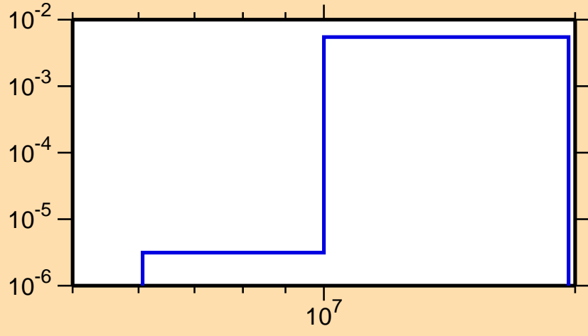
\sigma vs. E for ^{49}\text{Sc}(n,d)
