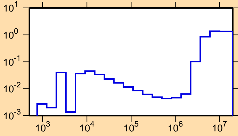
\sigma vs. E for ^{49}\text{Sc}(n,\text{nonel.})
