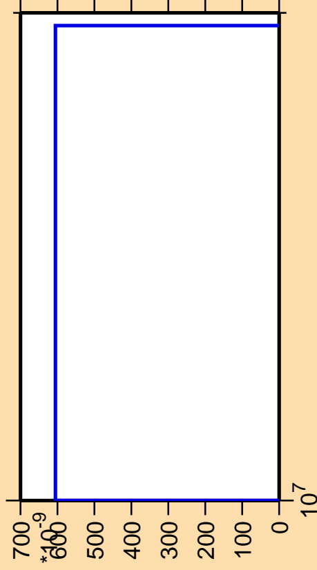
\Delta\sigma/\sigma vs. E for ^{49}\text{Sc}(n,\text{He}3)
