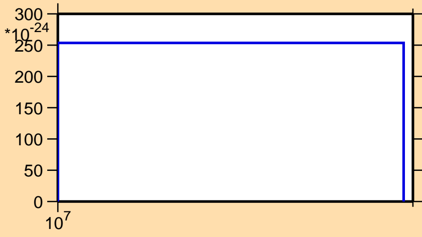
\sigma vs. E for ^{49}\text{Sc}(n,p\alpha)
