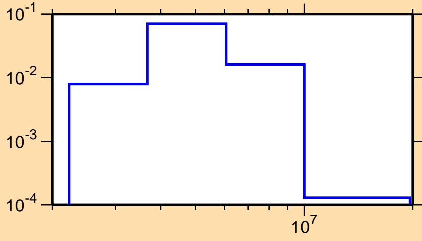
\sigma vs. E for ^{49}\text{Sc}(n,n_4)
