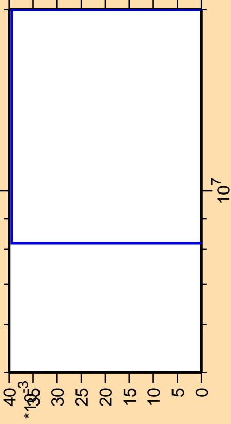
\Delta\sigma/\sigma vs. E for ^{49}\text{Sc}(n,nt)
