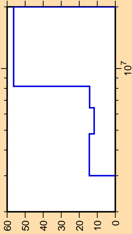
\Delta\sigma/\sigma vs. E for ^{50}\text{Sc}(n,\text{ncont.})
