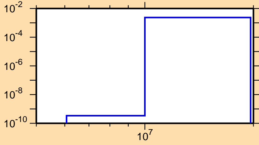
\sigma vs. E for ^{51}\text{Sc}(n,d)
