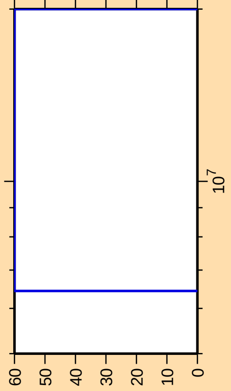
\Delta\sigma/\sigma vs. E for ^{52}\text{Sc}(n,\alpha)
