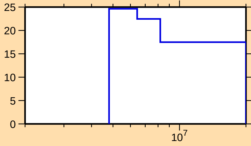
\Delta\sigma/\sigma vs. E for ^{52}\text{Sc}(n,2n)
