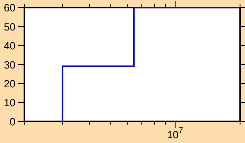
\Delta\sigma/\sigma vs. E for ^{52}\text{Sc}(n,n\text{cont.})
