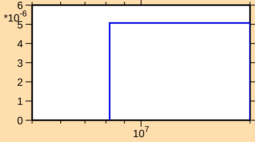
\sigma vs. E for ^{52}\text{Sc}(n,np)
