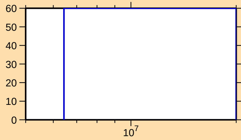
\Delta\sigma/\sigma vs. E for ^{52}\text{Sc}(n,n\text{cont.})
