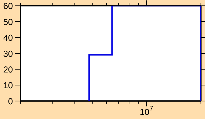
\Delta\sigma/\sigma vs. E for ^{52}\text{Sc}(n,ncont.)
