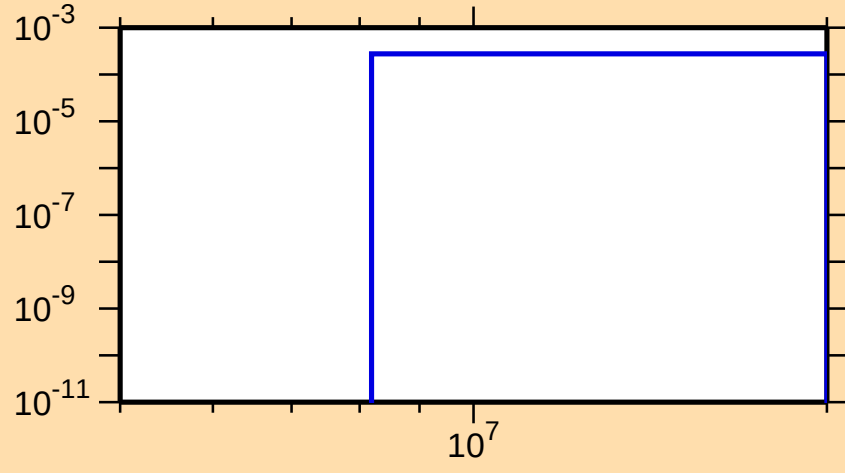
\sigma vs. E for ^{52}\text{Sc}(n,t)
