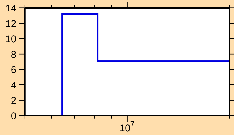
\Delta\sigma/\sigma vs. E for ^{52}\text{Sc}(n,\text{nonel.})
