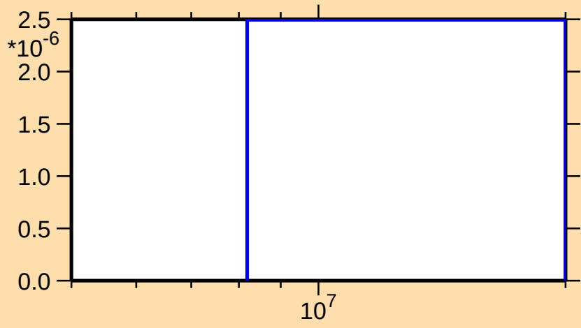
\sigma vs. E for ^{52}\text{Sc}(n,n\alpha)
