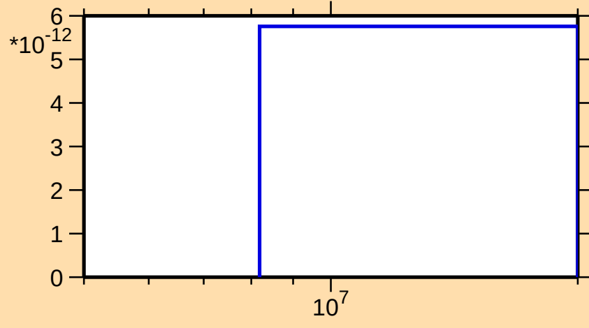
\sigma vs. E for ^{52}\text{Sc}(n,2n\alpha)
