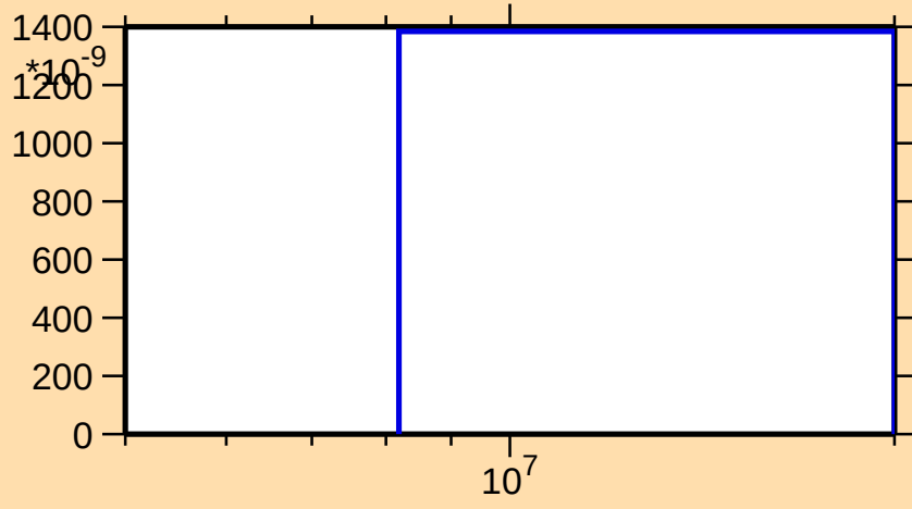
\sigma vs. E for ^{52}\text{Sc}(n,\text{nd})
