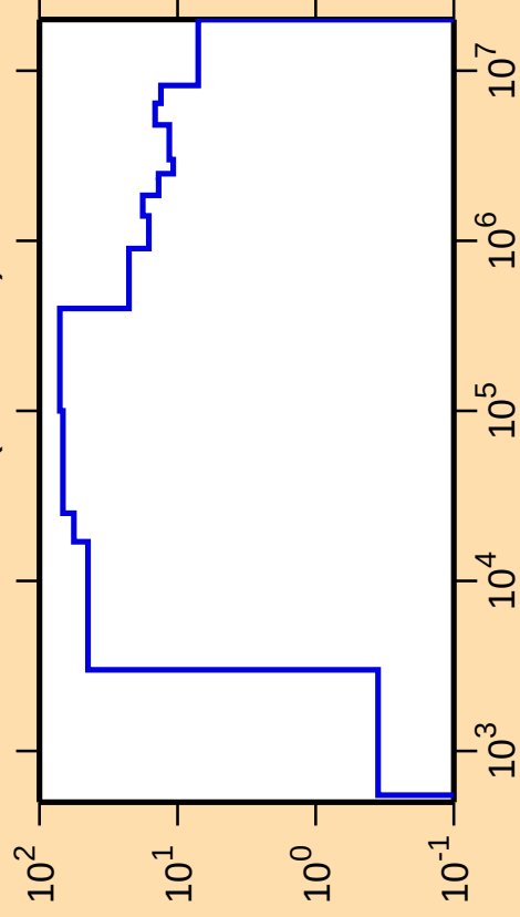
\Delta\sigma/\sigma vs. E for ^{52}\text{Sc}(n,\text{nonel.})
