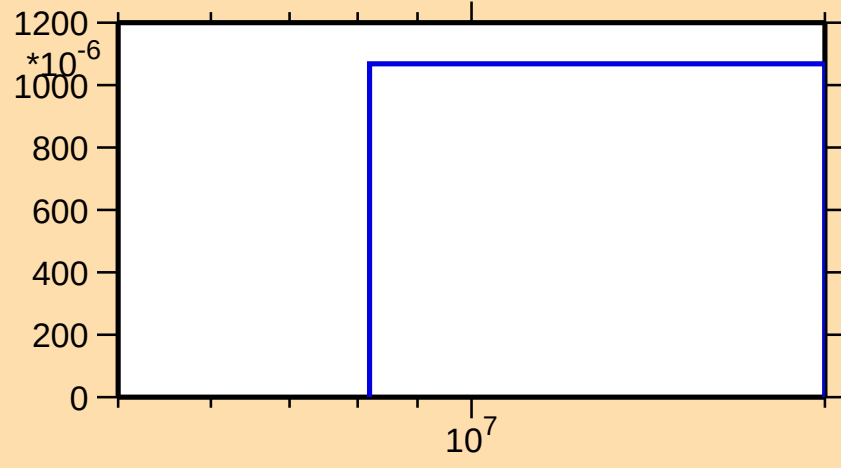
\sigma vs. E for ^{52}\text{Sc}(n,d)
