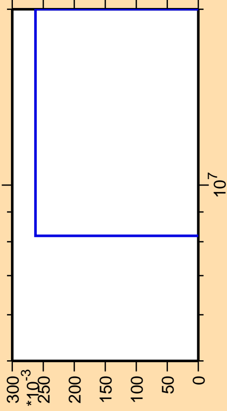
\Delta\sigma/\sigma vs. E for ^{53}\text{Sc}(n,2np)
