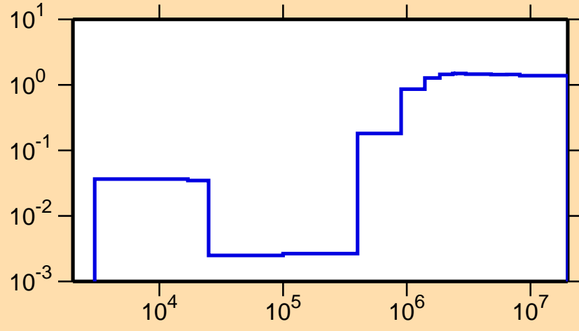
\sigma vs. E for ^{53}\text{Sc}(n,\text{nonel.})
