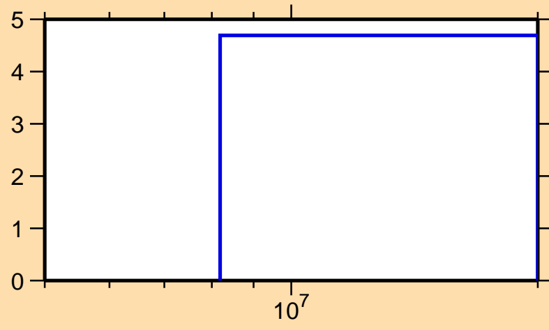
\Delta\sigma/\sigma vs. E for ^{53}\text{Sc}(n,\text{tot.})
