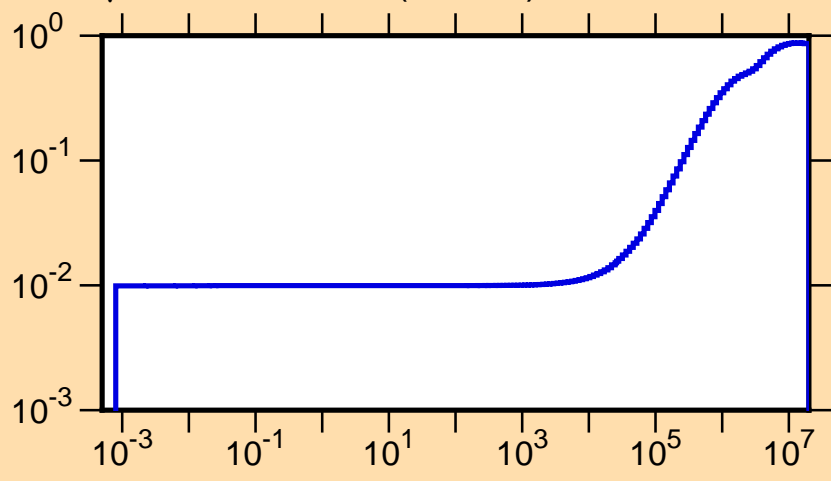
\mu vs. E for ^{68}\text{Se}(\text{mt251})
