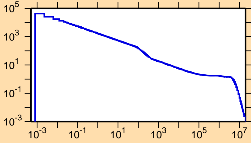
\sigma vs. E for ^{68}\text{Se}(n,p)
