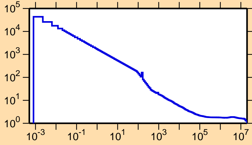
\sigma vs. E for ^{68}\text{Se}(n,\text{nonel.})
