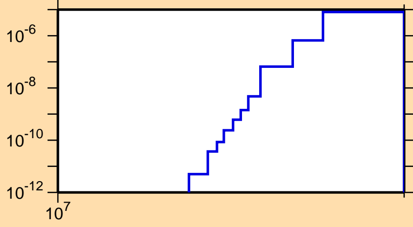
\sigma vs. E for ^{68}\text{Se} (mt 45)
