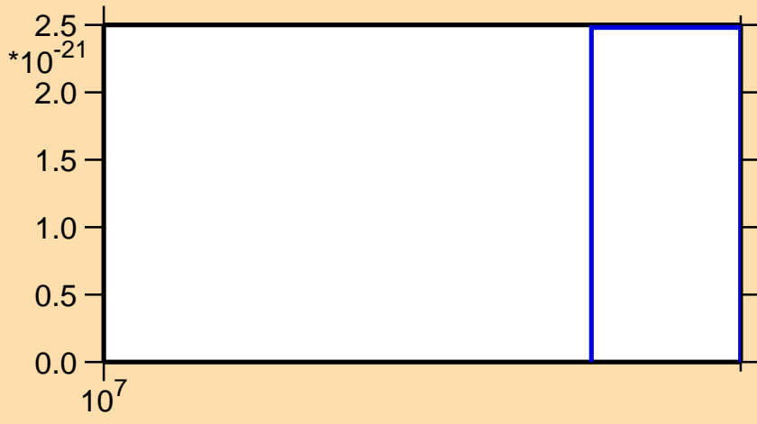
\sigma vs. E for ^{68}\text{Se}(n,2n\alpha)
