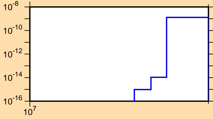
\sigma vs. E for ^{68}\text{Se}(n,\text{nd})
