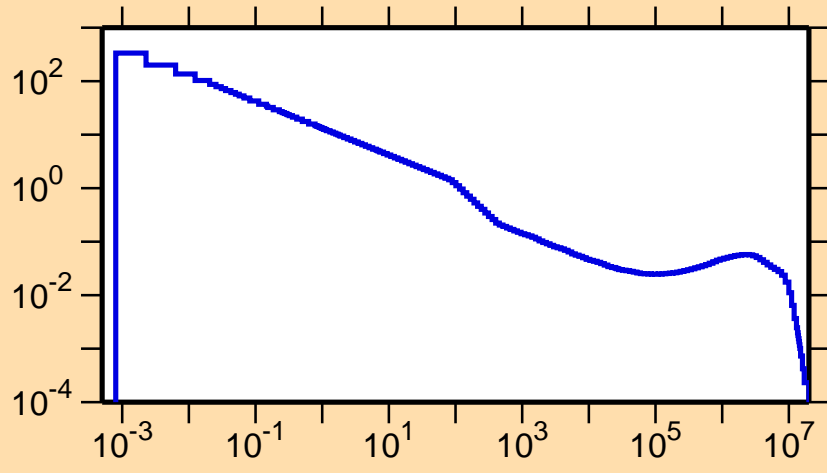
\sigma vs. E for ^{68}\text{Se}(n,\alpha)
