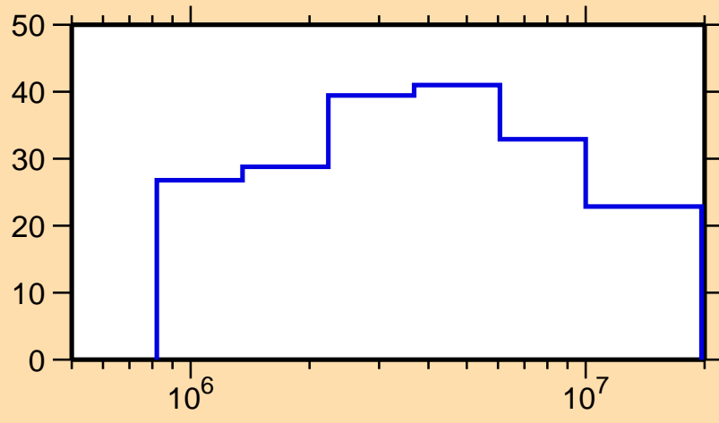
\Delta\sigma/\sigma vs. E for ^{68}\text{Se}(n,n_1)
