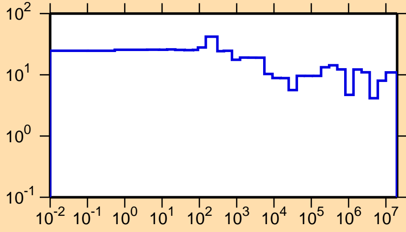
\Delta\sigma/\sigma vs. E for ^{68}\text{Se}(n,el.)
