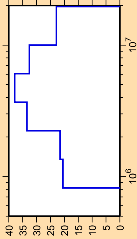
\Delta\sigma/\sigma vs. E for ^{68}\text{Se}(n,\text{inel.})
