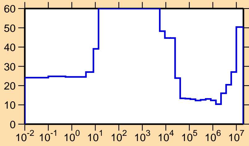
\Delta\sigma/\sigma vs. E for ^{68}\text{Se}(n,p)
