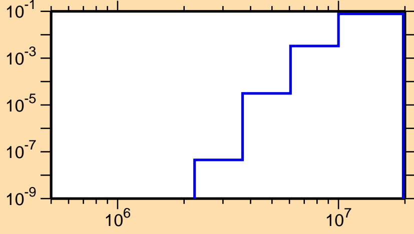
\sigma vs. E for ^{68}\text{Se}(n, p\alpha)
