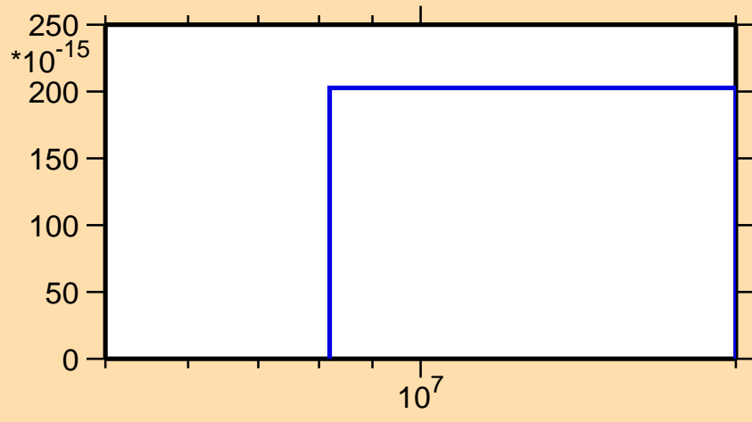
\sigma vs. E for ^{68}\text{Se}(n,2np)
