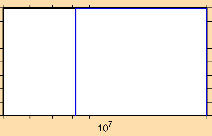
\sigma vs. E for ^{68}\text{Se}(\text{mt } 34)
