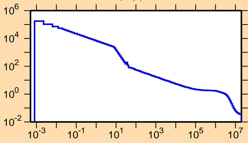
\sigma vs. E for ^{69}\text{Se}(n,p)
