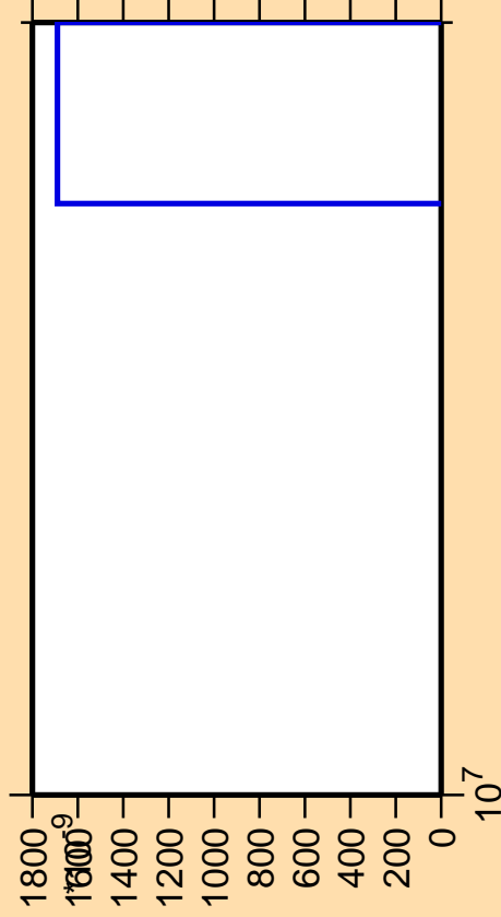
\Delta\sigma/\sigma vs. E for ^{69}\text{Se}(n,nt)
