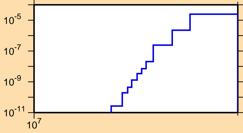
\sigma vs. E for ^{69}\text{Se} (mt 45)
