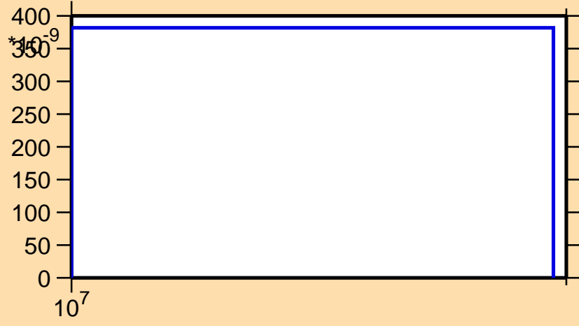
\sigma vs. E for ^{69}\text{Se} (mt 45)
