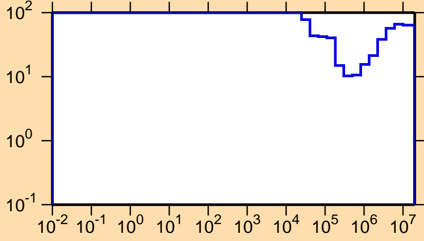
\Delta\sigma/\sigma vs. E for ^{69}\text{Se}(n,p)
