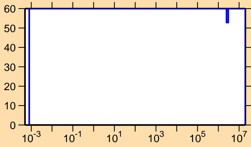
\Delta\sigma/\sigma vs. E for ^{69}\text{Se}(n,\gamma)
