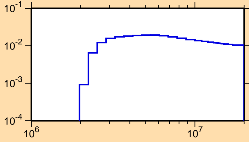
\sigma vs. E for ^{70}\text{Se}(n,n_4)
