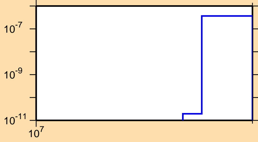
\sigma vs. E for ^{70}\text{Se}(n,pt)
