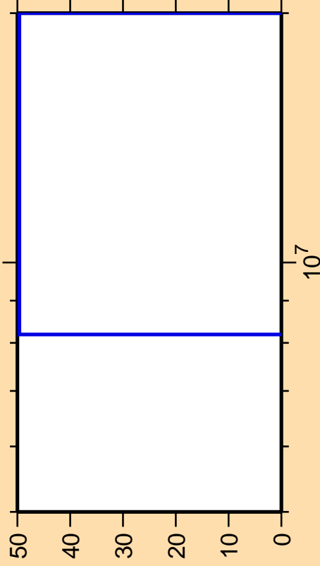
\Delta\sigma/\sigma vs. E for ^{70}\text{Se}(n,n\text{cont.})
