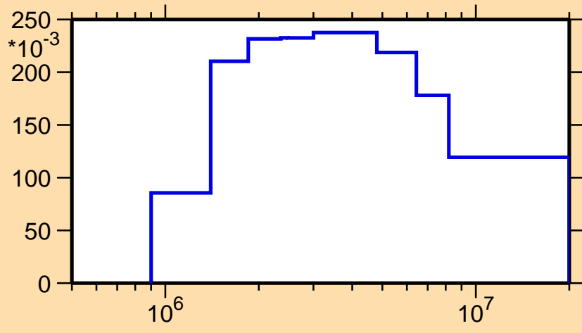
\sigma vs. E for ^{70}\text{Se}(n,n_1)
