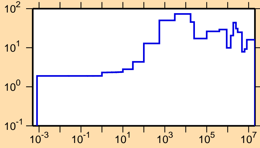
\Delta\sigma/\sigma vs. E for ^{70}\text{Se}(n,el.)
