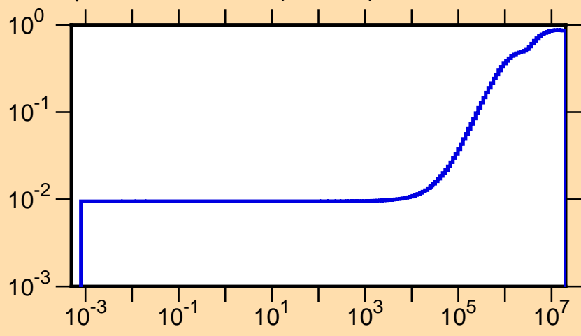
\mu vs. E for ^{71}\text{Se}(\text{mt251})
