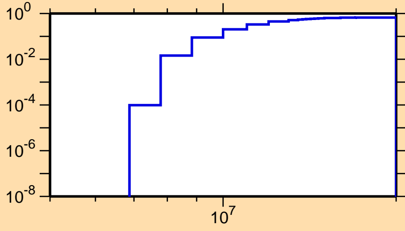
\sigma vs. E for ^{71}\text{Se}(n,np)
