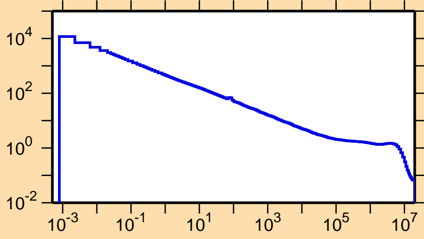
\sigma vs. E for ^{71}\text{Se}(n,p)
