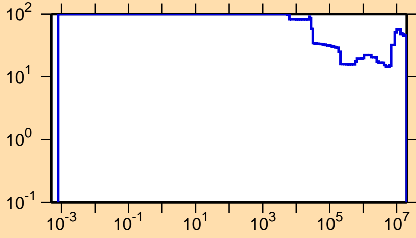
\Delta\sigma/\sigma vs. E for ^{71}\text{Se}(n,p)
