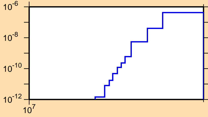
\sigma vs. E for ^{71}\text{Se}(\text{mt117})
