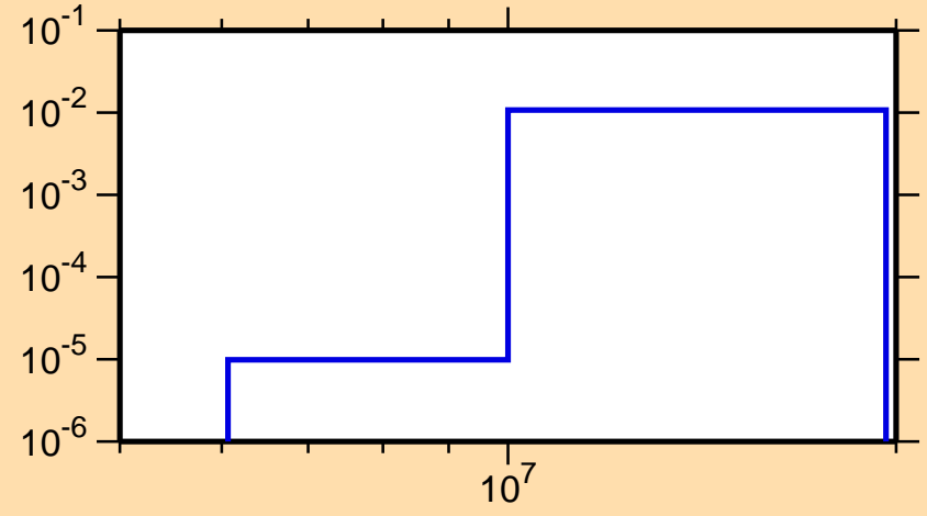
\sigma vs. E for ^{71}\text{Se}(n,2n)
