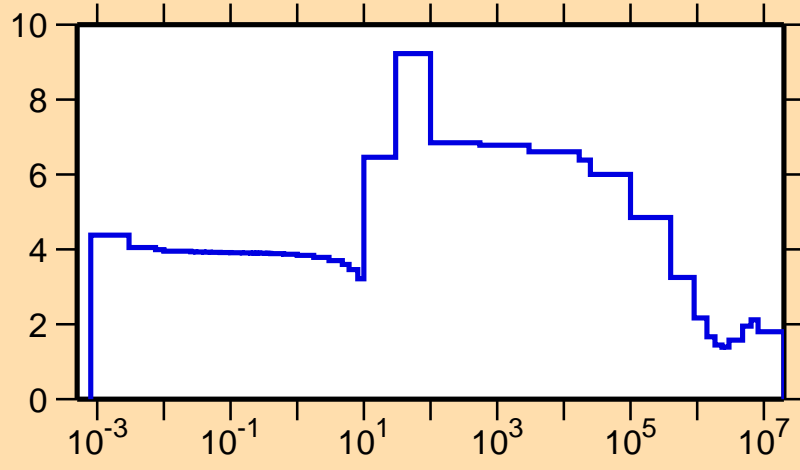
\sigma vs. E for ^{71}\text{Se}(n,\text{el.})
