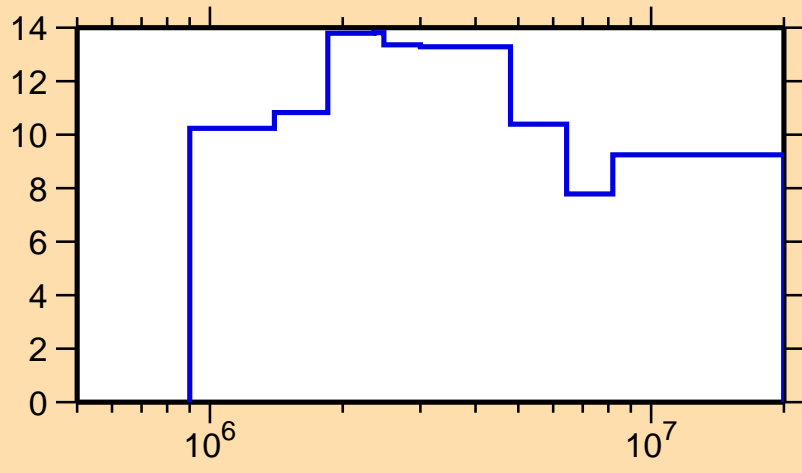
\Delta\sigma/\sigma vs. E for ^{71}\text{Se}(n,n\text{onel.})
