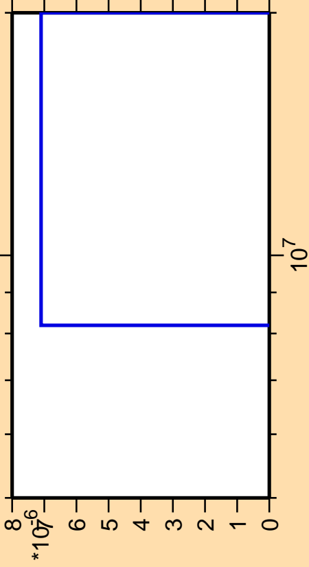
\Delta\sigma/\sigma vs. E for ^{71}\text{Se}(n,nt)
