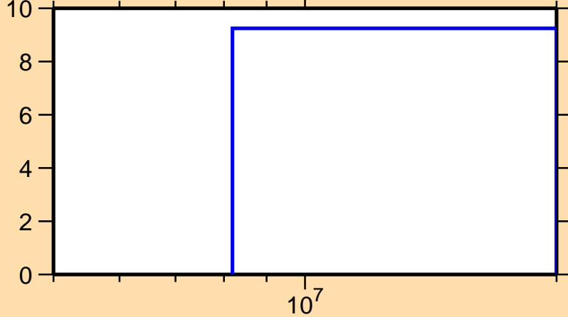
\Delta\sigma/\sigma vs. E for ^{71}\text{Se}(n,\text{nonel.})
