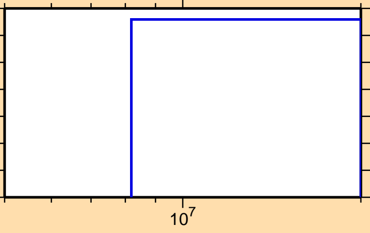
\sigma vs. E for ^{71}\text{Se}(n,2np)
