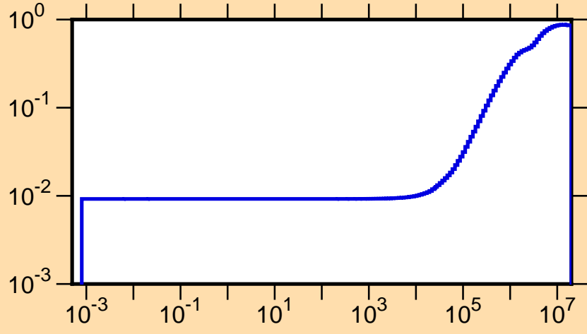
\mu vs. E for ^{73}\text{Se}(\text{mt251})
