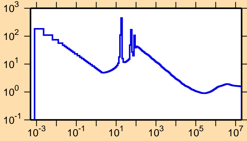
\sigma vs. E for ^{73}\text{Se}(n,\text{nonel.})
