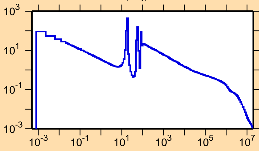
\sigma vs. E for ^{73}\text{Se}(n,\gamma)
