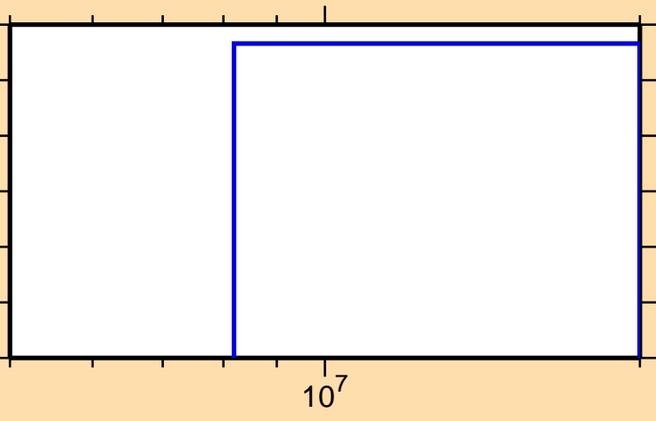
\sigma vs. E for ^{73}\text{Se}(n,\text{pd})
