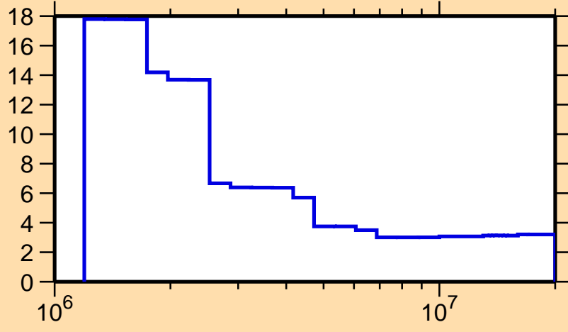
\Delta\sigma/\sigma vs. E for ^{73}\text{Se}(n,n\text{onel.})
