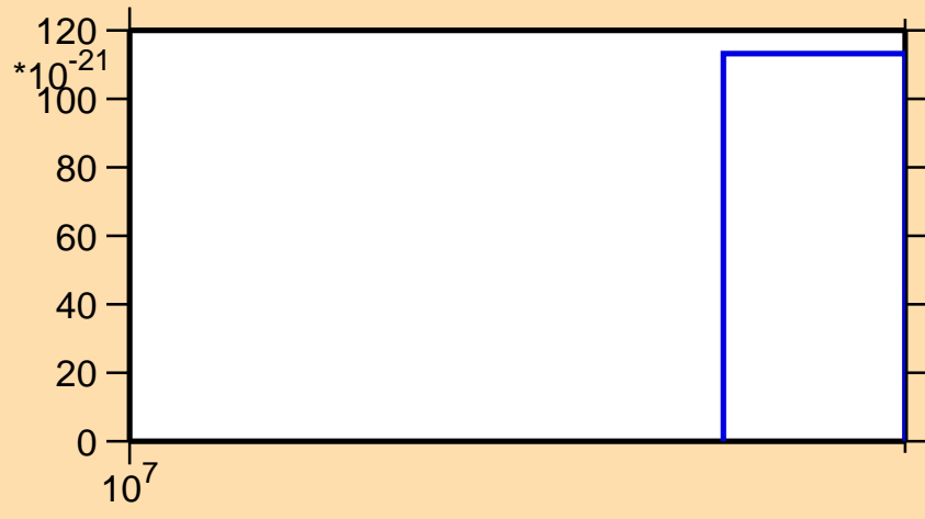
\sigma vs. E for ^{73}\text{Se}(n,nt)
