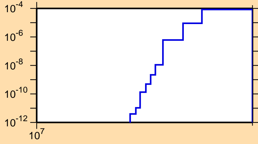
\sigma vs. E for ^{73}\text{Se}(n,pd)
