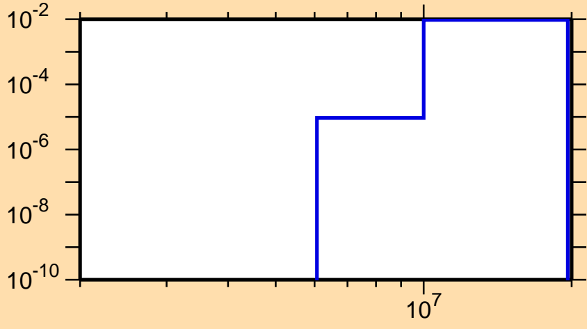
\sigma vs. E for ^{73}\text{Se}(n,d)
