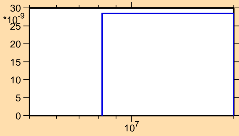
\sigma vs. E for ^{73}\text{Se}(n,pt)
