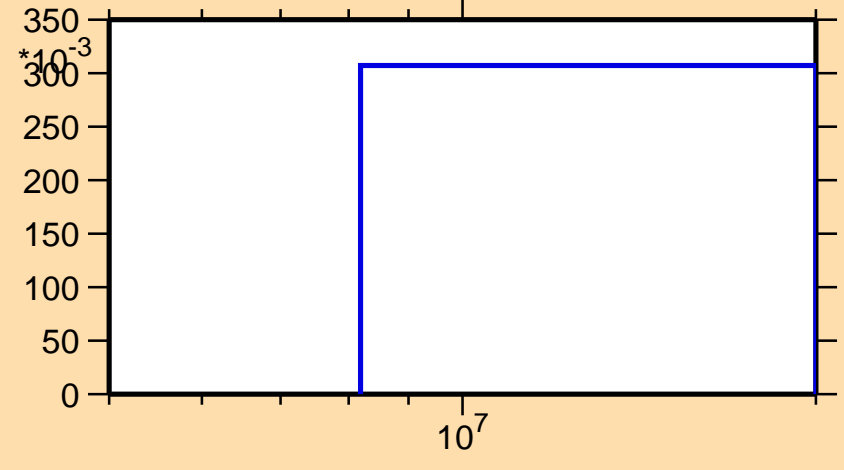
\sigma vs. E for ^{73}\text{Se}(n,2n)
