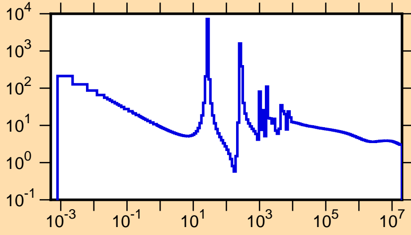
\sigma vs. E for ^{74}\text{Se}(n,\text{tot.})
