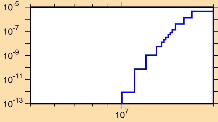
\sigma vs. E for ^{74}\text{Se}(n,\text{He}3)
