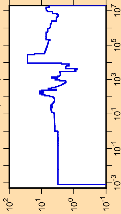
\Delta\sigma/\sigma vs. E for ^{74}\text{Se}(n,\text{tot.})
