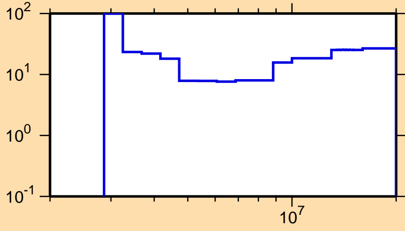
\Delta\sigma/\sigma vs. E for ^{74}\text{Se}(n,ncont.)
