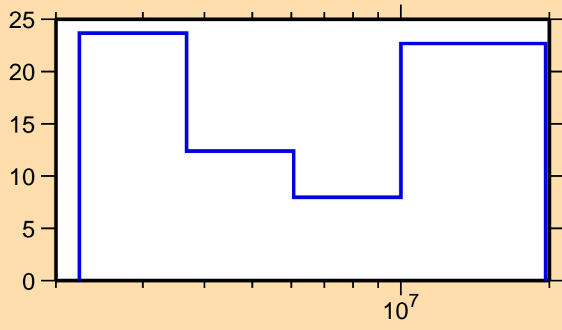
\Delta\sigma/\sigma vs. E for ^{74}\text{Se}(n,ncont.)
