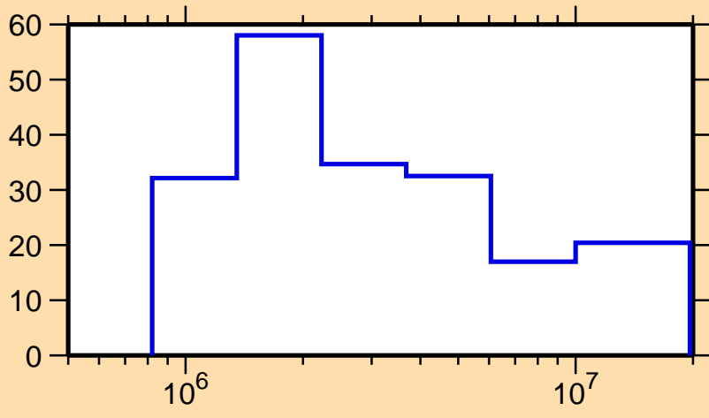
\Delta\sigma/\sigma vs. E for ^{74}\text{Se}(n,p)
