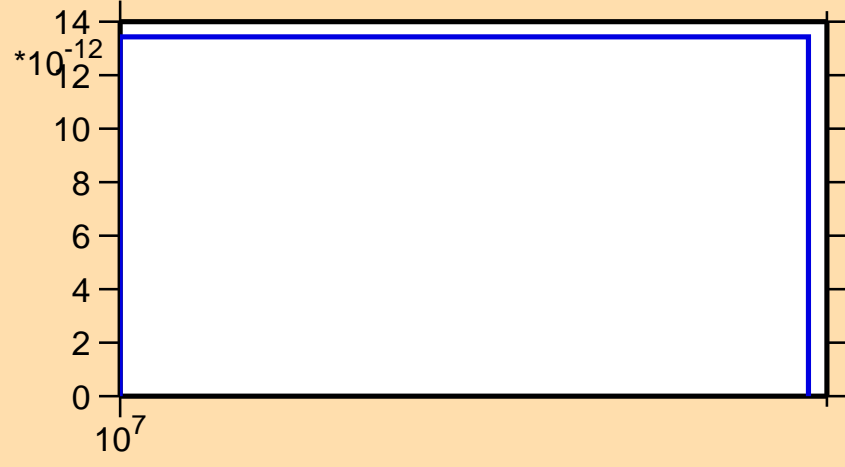
\sigma vs. E for ^{74}\text{Se}(n,nd)
