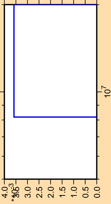
\Delta\sigma/\sigma vs. E for ^{74}\text{Se}(n,2np)
