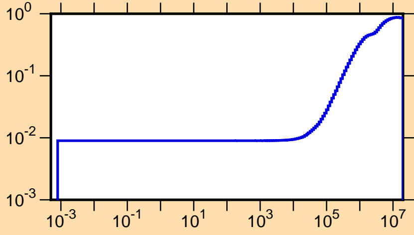
\mu vs. E for ^{75}\text{Se}(\text{mt251})
