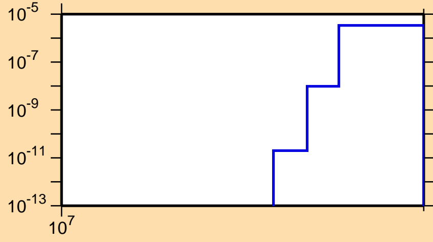
\sigma vs. E for ^{75}\text{Se}(n,2n\alpha)
