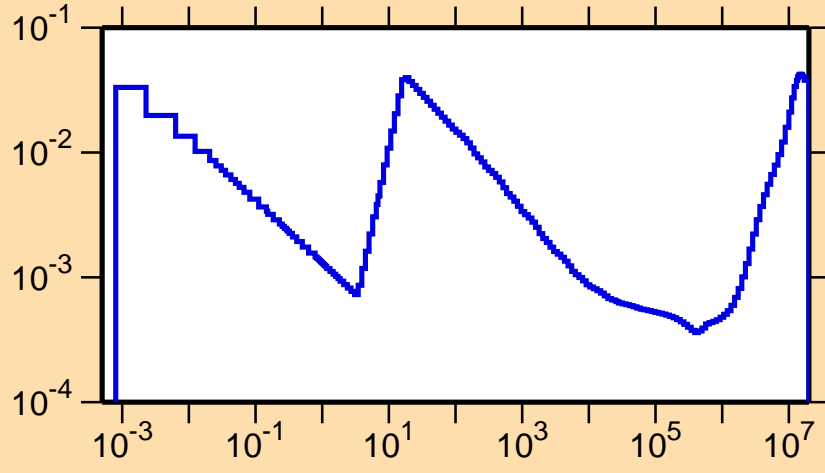
\sigma vs. E for ^{75}\text{Se}(n,\alpha)
