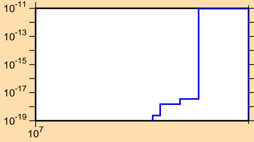
\sigma vs. E for ^{75}\text{Se} (mt 34)
