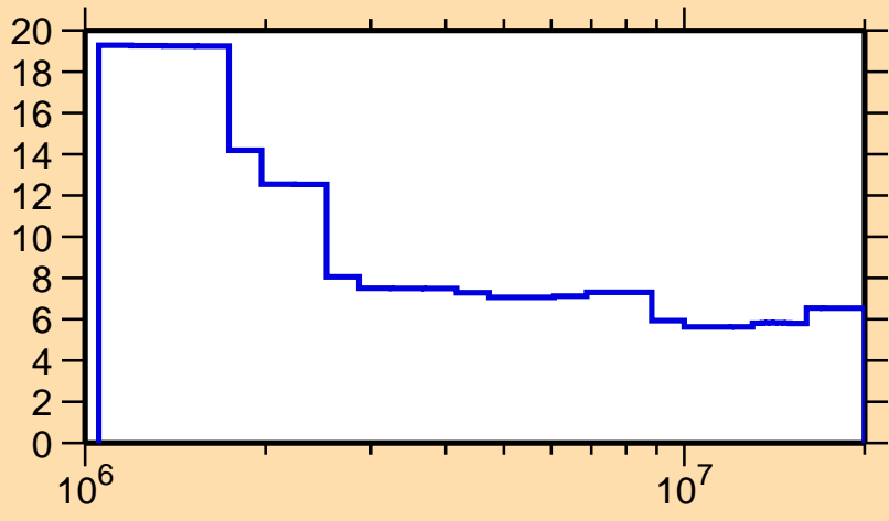
\Delta\sigma/\sigma vs. E for ^{75}\text{Se}(n,n\text{onel.})
