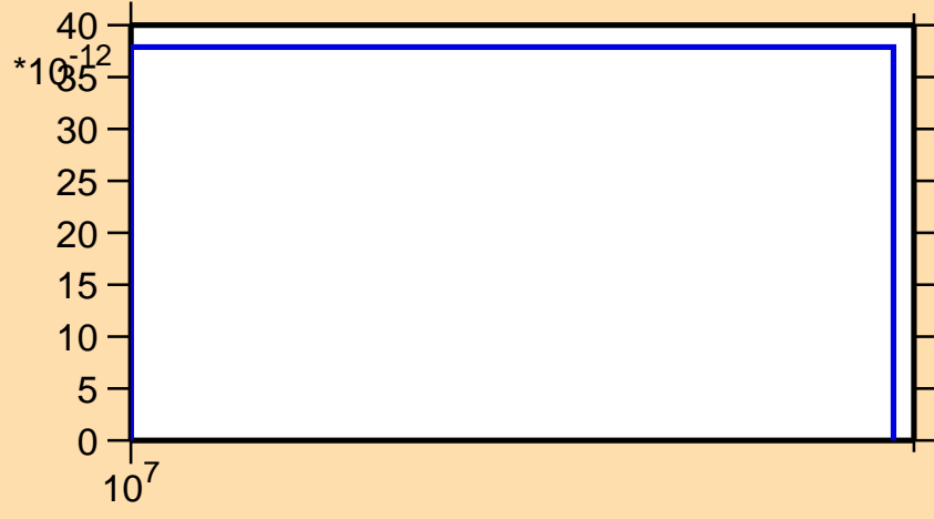
\sigma vs. E for ^{75}\text{Se}(n,pd)
