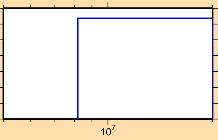
\sigma vs. E for ^{75}\text{Se}(n,\text{pt})
