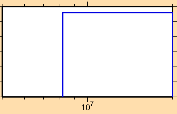
\sigma vs. E for ^{75}\text{Se}(n,2n\alpha)
